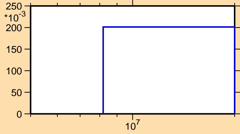
\sigma vs. E for ^{133}\text{Pr}(n,2n)
