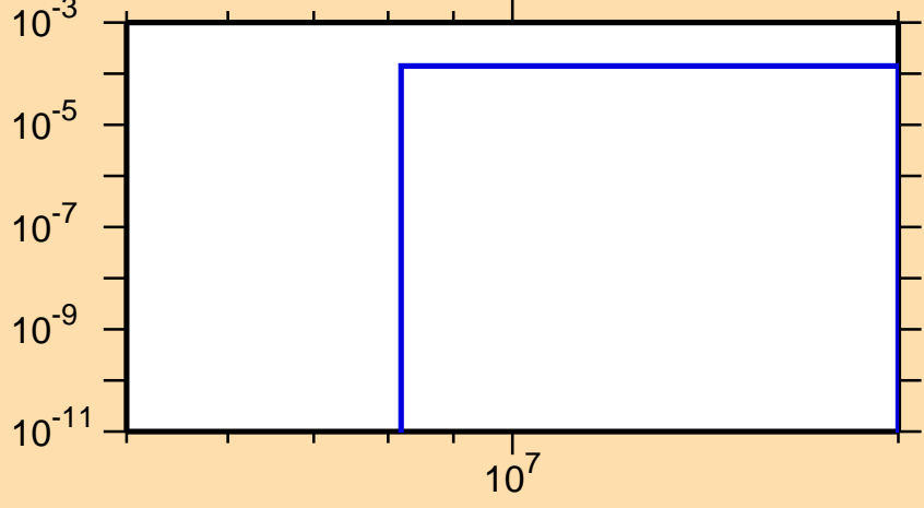
\sigma vs. E for ^{133}\text{Pr}(n,t)
