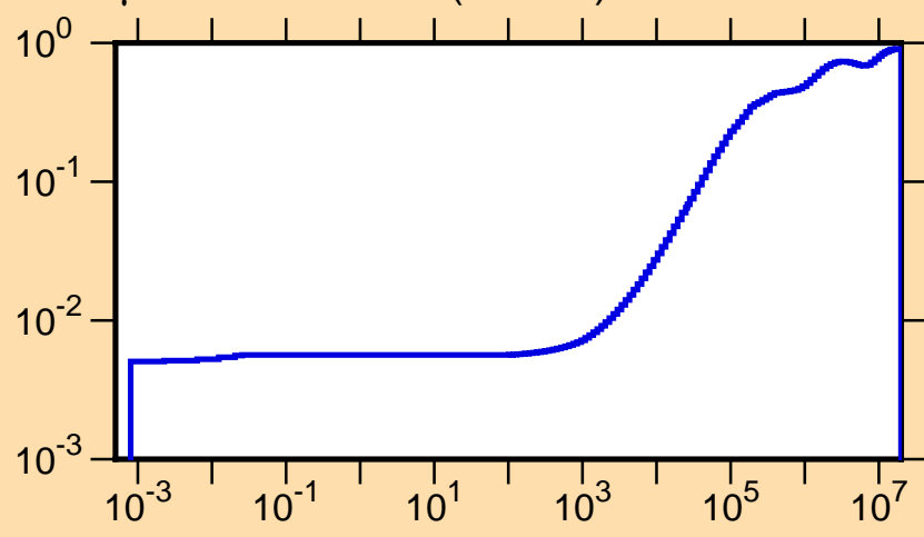
\mu vs. E for ^{134}\text{Pr}(\text{mt251})
