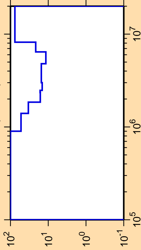
\Delta\sigma/\sigma vs. E for ^{134}\text{Pr}(n,\text{inel.})
