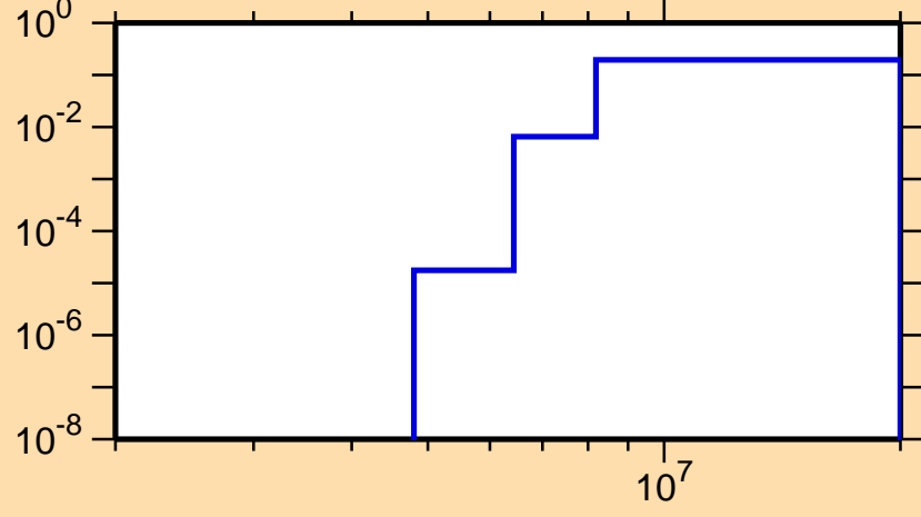
\sigma vs. E for ^{134}\text{Pr}(n,np)
