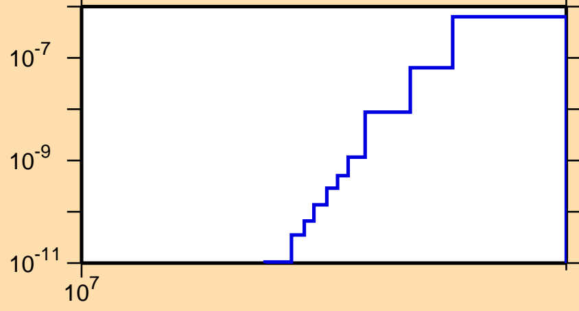
\sigma vs. E for ^{134}\text{Pr}(\text{mt } 45)
