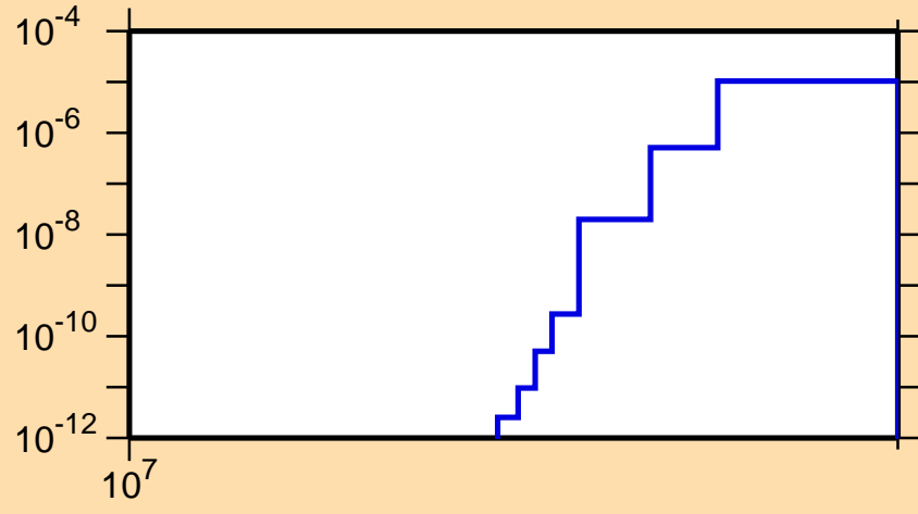
\sigma vs. E for ^{135}\text{Pr}(n,nd)
