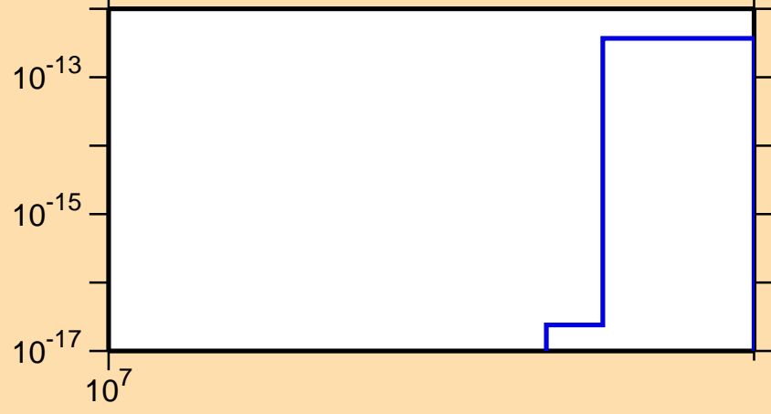
\sigma vs. E for ^{135}\text{Pr}(\text{mt } 34)
