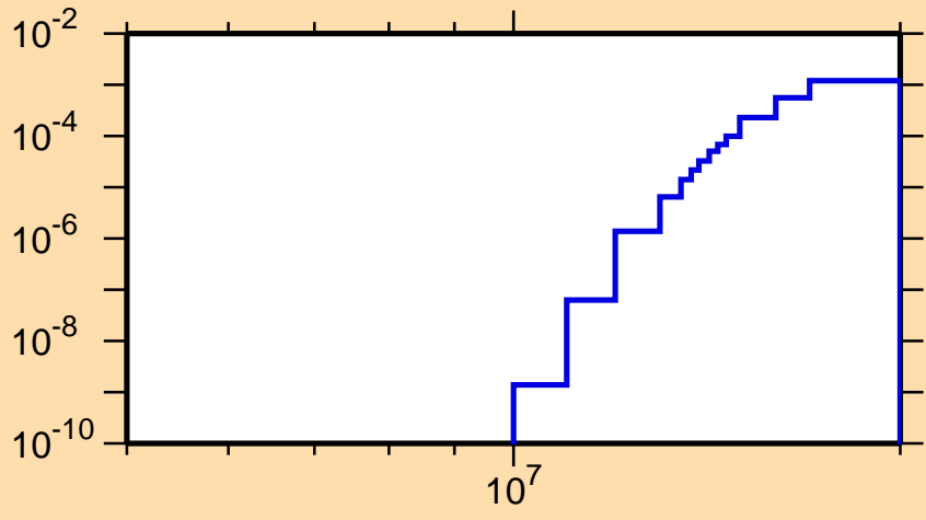
\sigma vs. E for ^{135}\text{Pr}(n,t)
