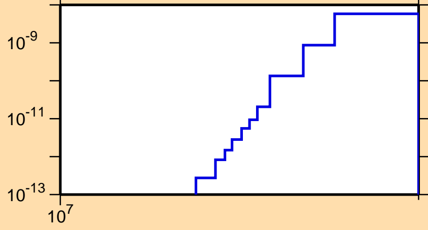
\sigma vs. E for ^{135}\text{Pr}(\text{mt117})
