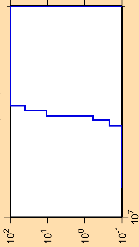
\Delta\sigma/\sigma vs. E for ^{135}\text{Pr}(n,nd)
