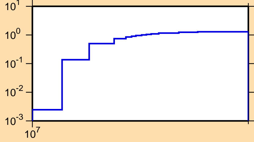
\sigma vs. E for ^{135}\text{Pr}(n,2n)
