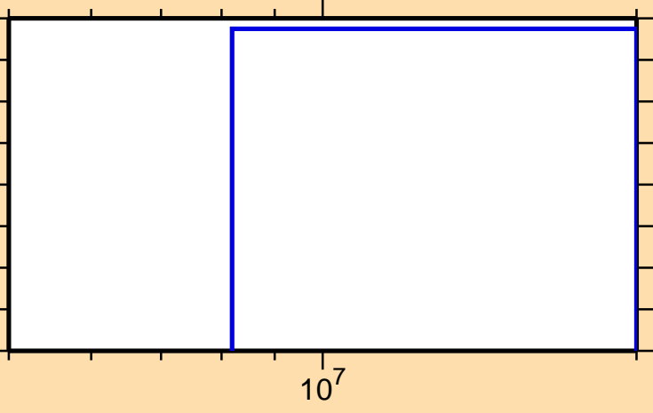
\sigma vs. E for ^{135}\text{Pr}(n,t)
