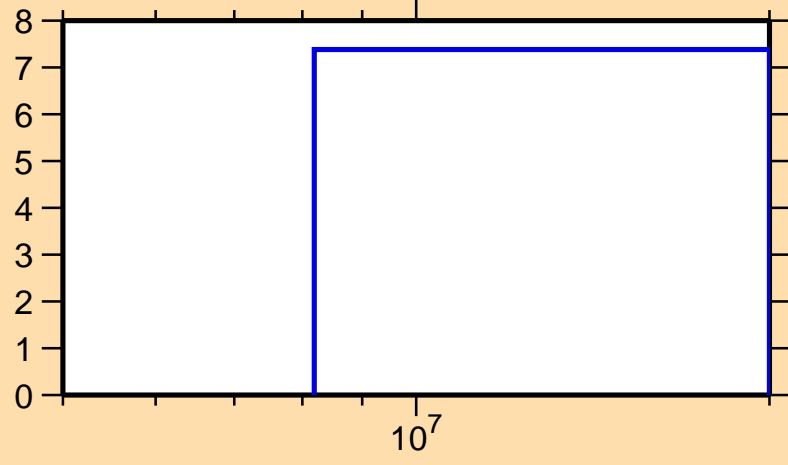
\Delta\sigma/\sigma vs. E for ^{135}\text{Pr}(n,\text{el.})
