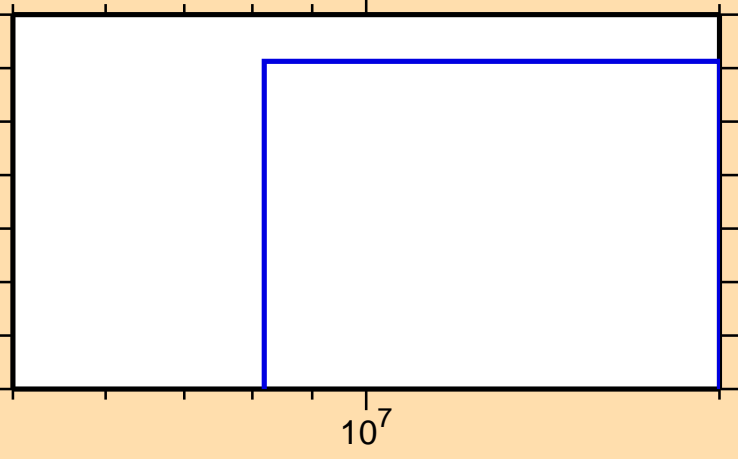
\sigma vs. E for ^{135}\text{Pr}(n,\text{pd})
