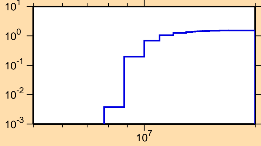
\sigma vs. E for ^{136}\text{Pr}(n,2n)
