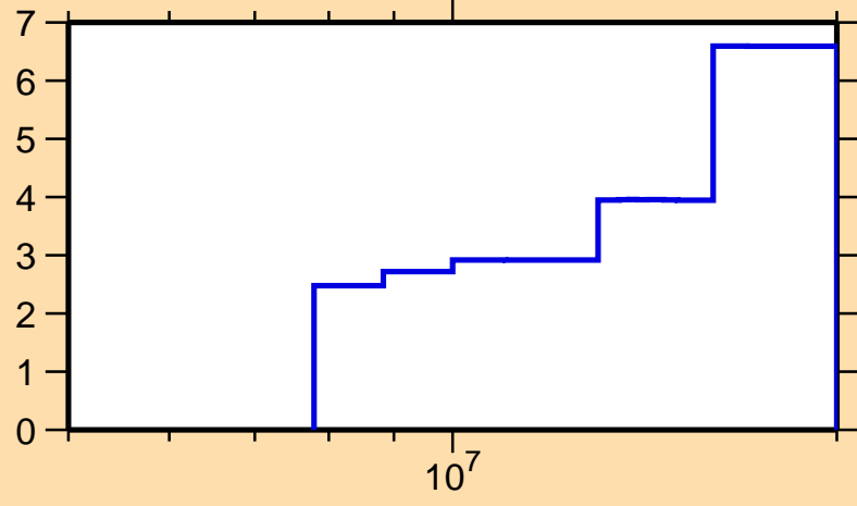
\Delta\sigma/\sigma vs. E for ^{136}\text{Pr}(n,\text{el.})
