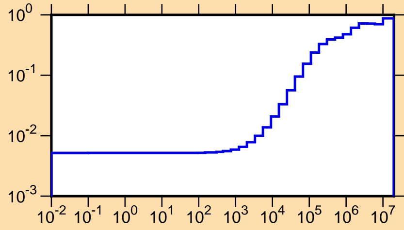
\mu vs. E for ^{136}\text{Pr}(\text{mt251})
