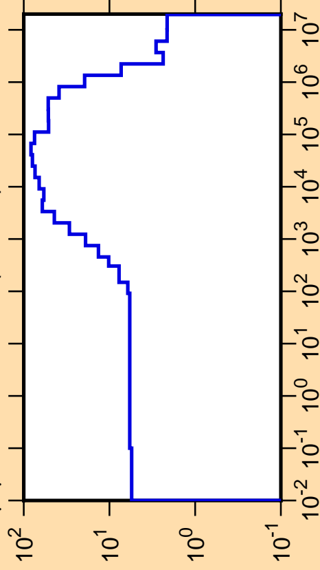
\Delta\mu/\mu vs. E for ^{136}\text{Pr}(\text{mt251})
