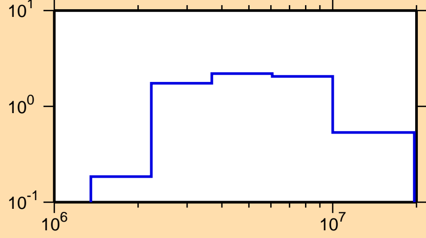
\sigma vs. E for ^{136}\text{Pr}(n,n\text{cont.})
