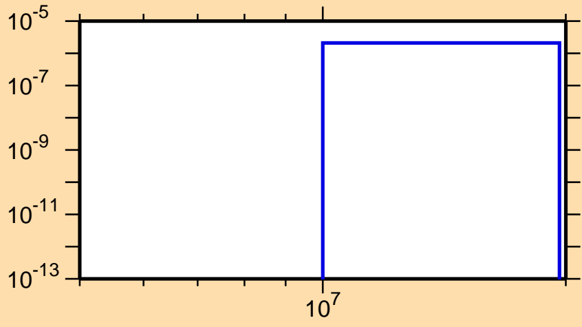
\sigma vs. E for ^{136}\text{Pr}(n,\text{nd})
