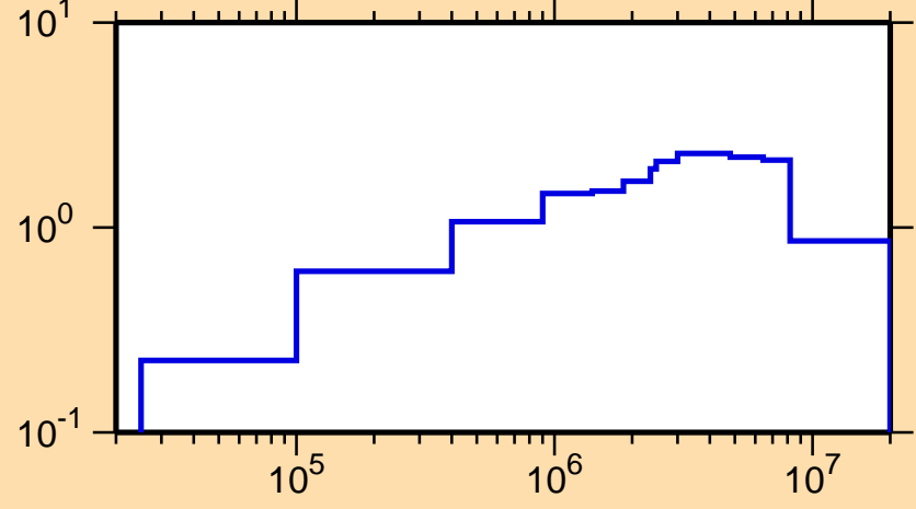
\sigma vs. E for ^{136}\text{Pr}(n,\text{inel.})
