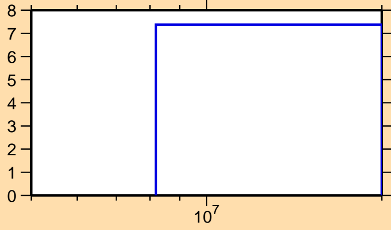
\Delta\sigma/\sigma vs. E for ^{136}\text{Pr}(n,2n)
