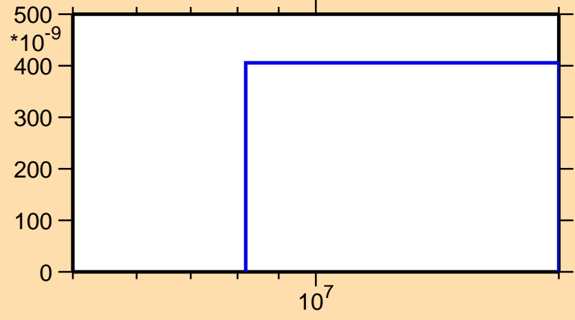
\sigma vs. E for ^{136}\text{Pr}(n,\text{He}3)
