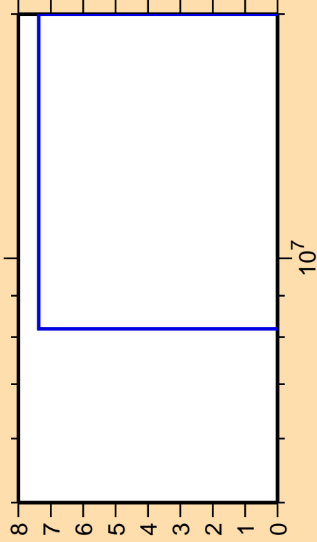
\Delta\sigma/\sigma vs. E for ^{136}\text{Pr}(n,2n)
