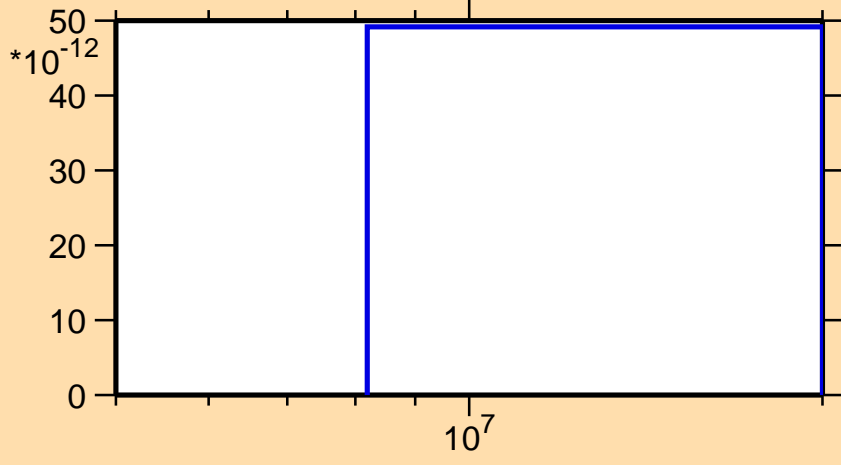
\sigma vs. E for ^{136}\text{Pr}(n,\text{pd})
