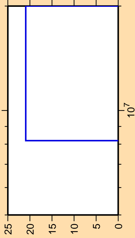
\Delta\sigma/\sigma vs. E for ^{136}\text{Pr}(n,\gamma)
