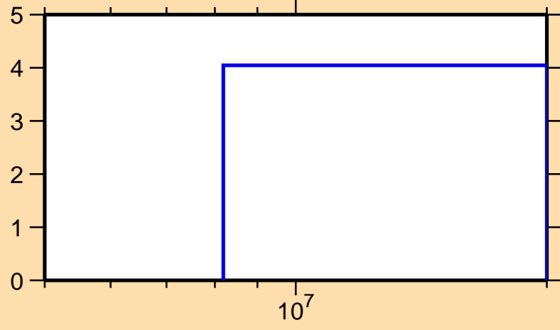
\Delta\sigma/\sigma vs. E for ^{136}\text{Pr}(n,\text{nonel.})
