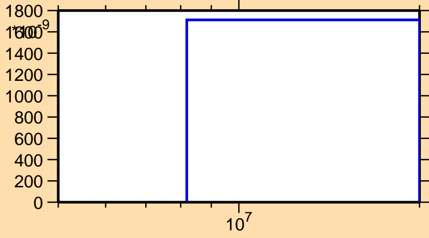
\sigma vs. E for ^{136}\text{Pr}(n,\text{nd})
