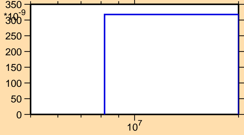
\sigma vs. E for ^{136}\text{Pr}(n,3n)
