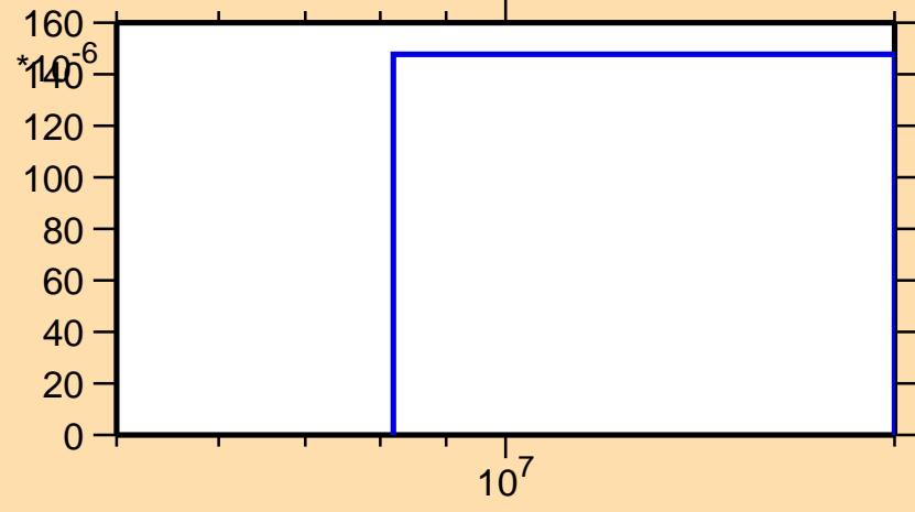
\sigma vs. E for ^{136}\text{Pr}(n,2np)
