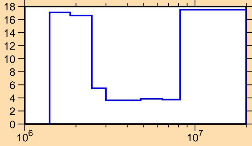
\Delta\sigma/\sigma vs. E for ^{136}\text{Pr}(n,n\text{cont.})
