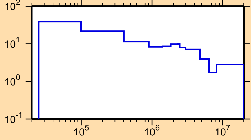
\Delta\sigma/\sigma vs. E for ^{136}\text{Pr}(n,\text{tot.})
