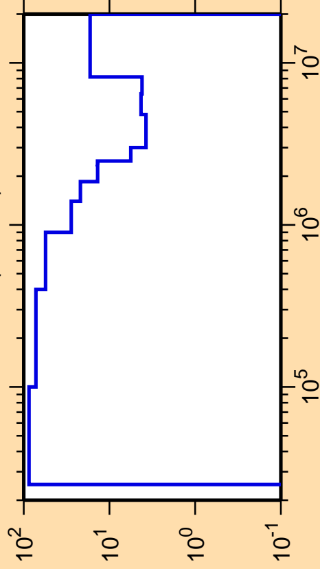
\Delta\sigma/\sigma vs. E for ^{136}\text{Pr}(n,\text{inel.})
