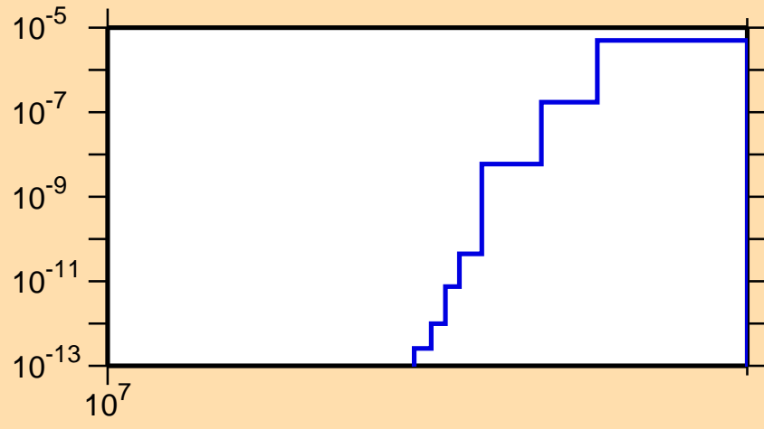
\sigma vs. E for ^{137}\text{Pr}(n,nd)
