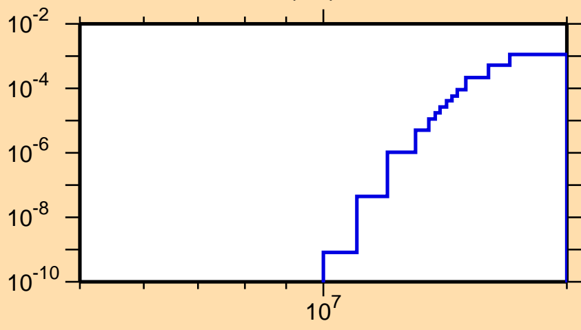
\sigma vs. E for ^{137}\text{Pr}(n,t)
