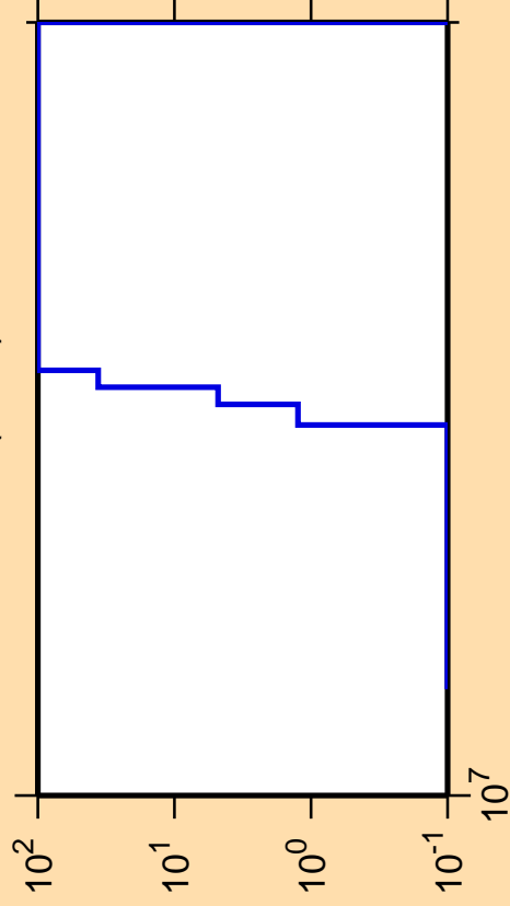
\Delta\sigma/\sigma vs. E for ^{137}\text{Pr}(n,nd)
