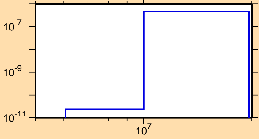
\sigma vs. E for ^{137}\text{Pr}(n,p\alpha)
