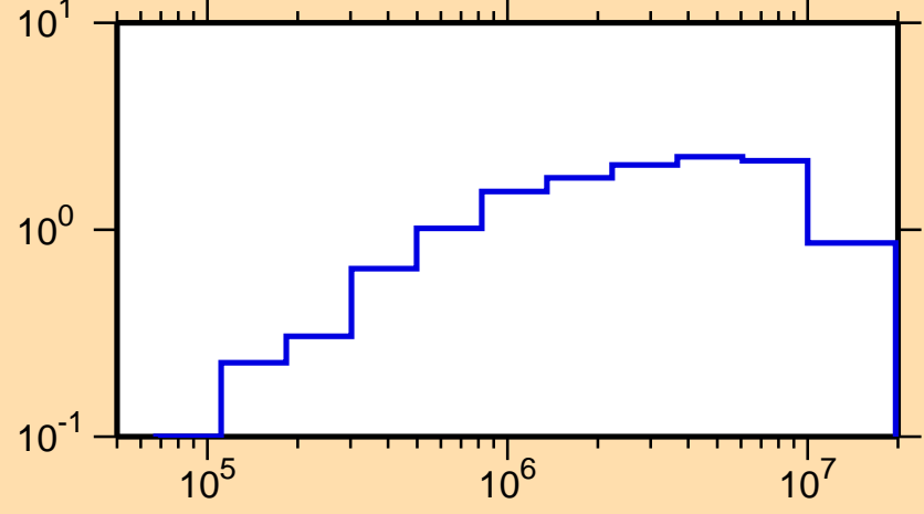
\sigma vs. E for ^{137}\text{Pr}(n,\text{inel.})
