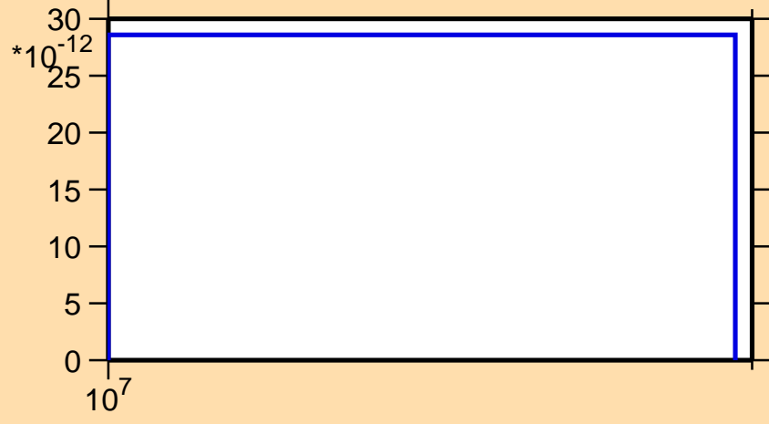
\sigma vs. E for ^{137}\text{Pr}(n,\text{pd})
