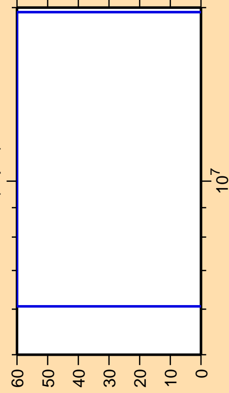
\Delta\sigma/\sigma vs. E for ^{137}\text{Pr}(n,p\alpha)
