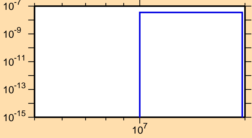
\sigma vs. E for ^{137}\text{Pr}(n,\text{He3})
