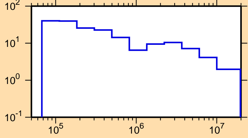
\Delta\sigma/\sigma vs. E for ^{137}\text{Pr}(n,\text{tot.})
