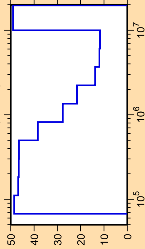
\Delta\sigma/\sigma vs. E for ^{137}\text{Pr}(n,\text{inel.})
