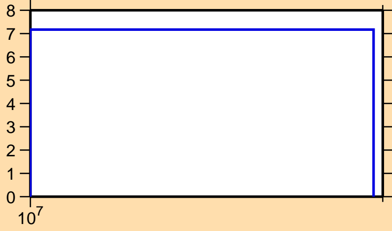
\Delta\sigma/\sigma vs. E for ^{137}\text{Pr}(n,el.)
