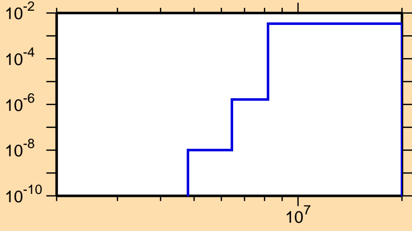
\sigma vs. E for ^{137}\text{Pr}(n,d)
