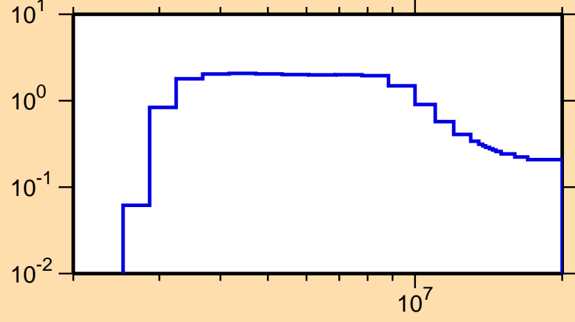
\sigma vs. E for ^{138}\text{Pr}(n,n\text{cont.})
