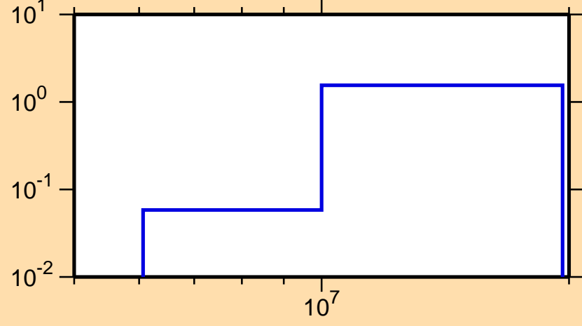
\sigma vs. E for ^{138}\text{Pr}(n,2n)
