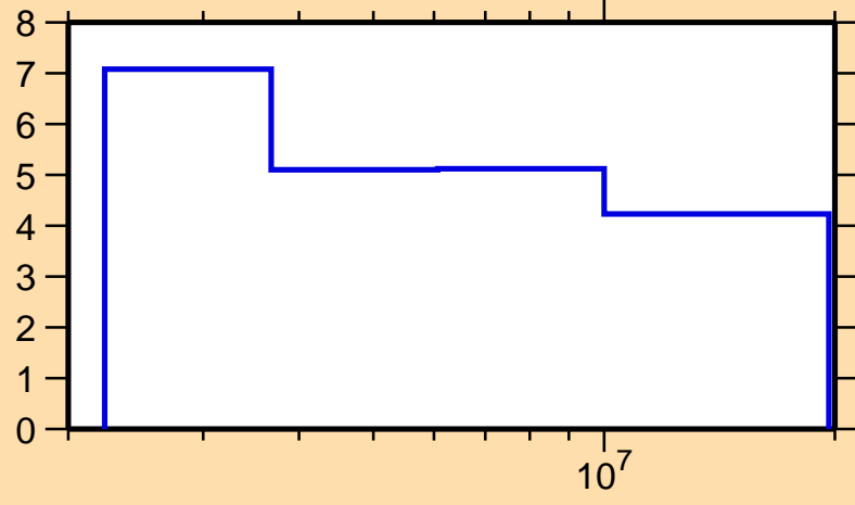
\Delta\sigma/\sigma vs. E for ^{138}\text{Pr}(n,n\text{onel.})
