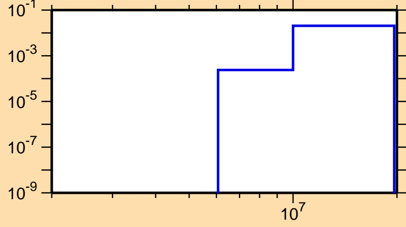
\sigma vs. E for ^{138}\text{Pr}(n,np)
