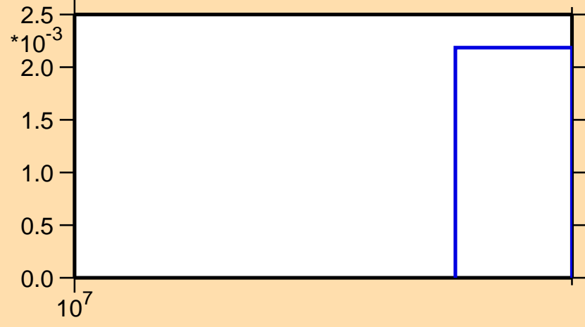
\sigma vs. E for ^{139}\text{Pr}(n,3n)
