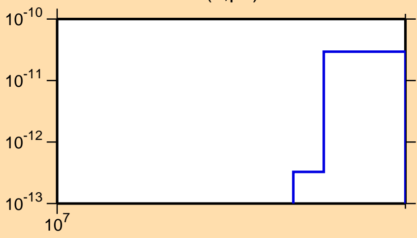
\sigma vs. E for ^{139}\text{Pr}(n,\text{pd})
