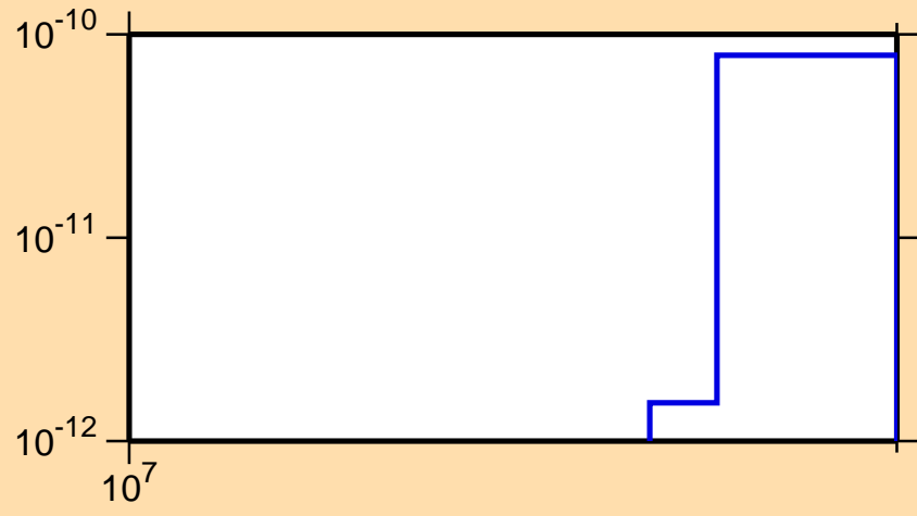
\sigma vs. E for ^{139}\text{Pr}(\text{mt } 45)
