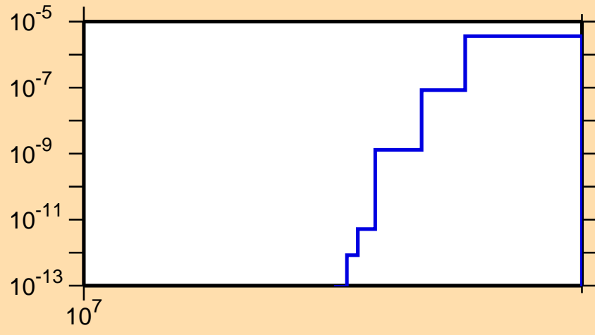
\sigma vs. E for ^{139}\text{Pr}(n,\text{nd})
