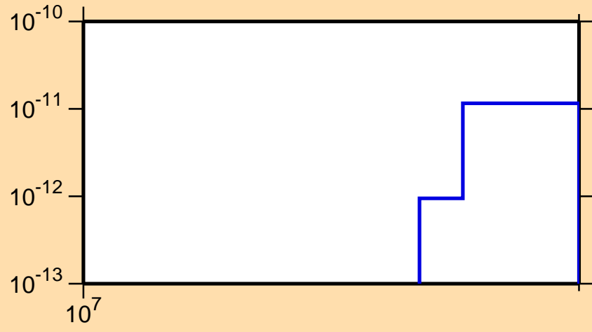
\sigma vs. E for ^{139}\text{Pr}(\text{mt117})
