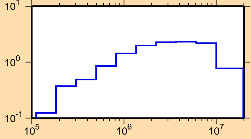
\sigma vs. E for ^{139}\text{Pr}(n,\text{inel.})
