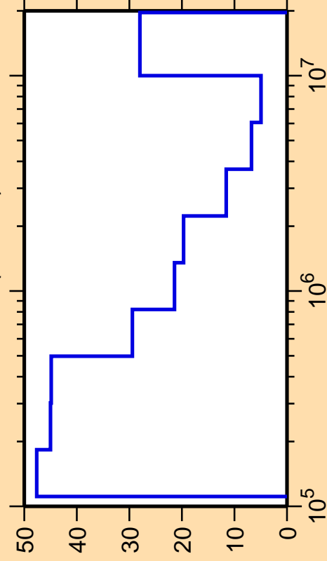
\Delta\sigma/\sigma vs. E for ^{139}\text{Pr}(n,\text{inel.})
