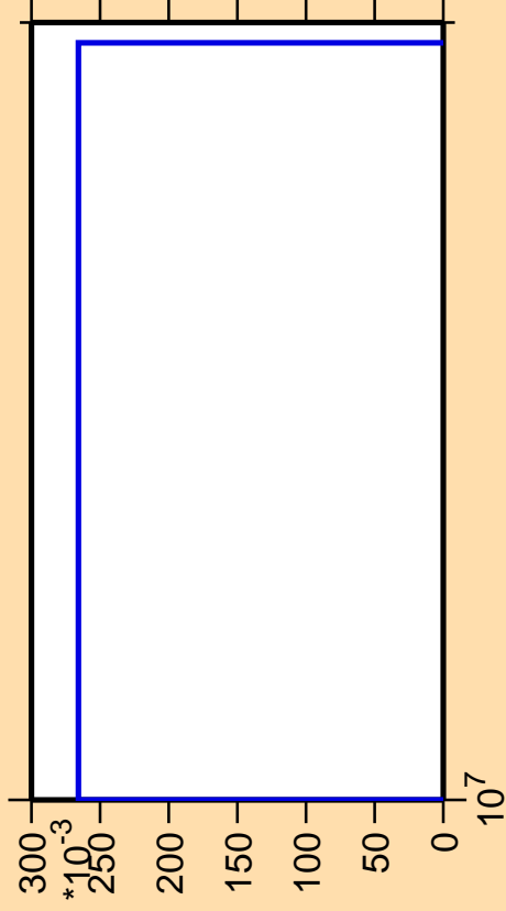
\Delta\sigma/\sigma vs. E for ^{139}\text{Pr}(n,\text{pd})
