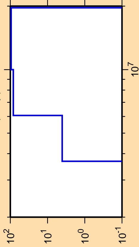
\Delta\sigma/\sigma vs. E for ^{139}\text{Pr}(n,np)
