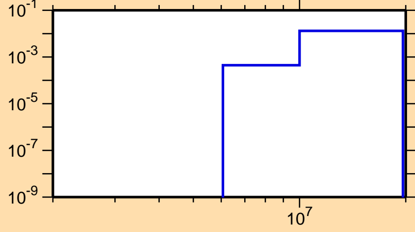
\sigma vs. E for ^{139}\text{Pr}(n,np)
