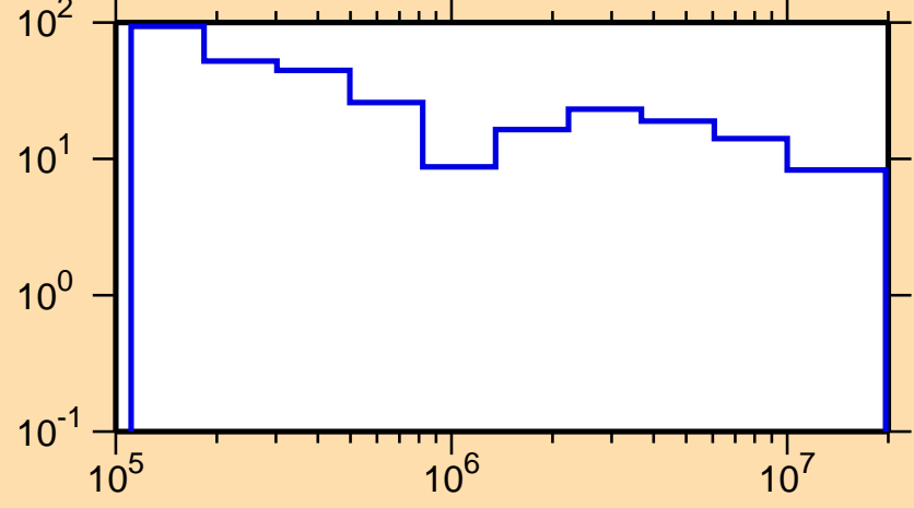
\Delta\sigma/\sigma vs. E for ^{139}\text{Pr}(n,\text{el.})
