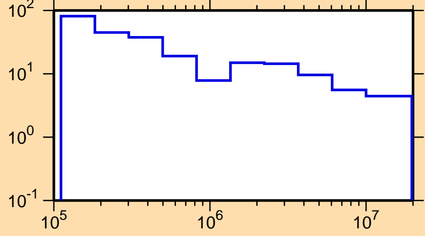
\Delta\sigma/\sigma vs. E for ^{139}\text{Pr}(n,\text{tot.})
