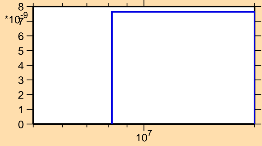
\sigma vs. E for ^{139}\text{Pr}(n,p\alpha)
