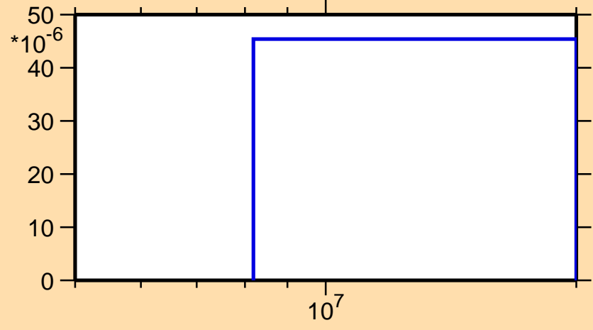
\sigma vs. E for ^{139}\text{Pr}(n,t)
