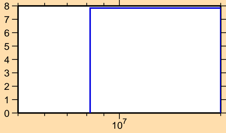
\Delta\sigma/\sigma vs. E for ^{139}\text{Pr}(n,\text{el.})
