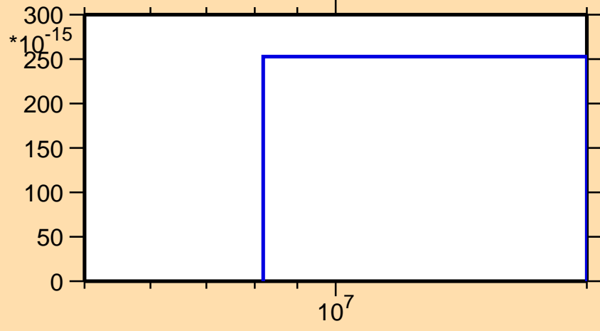
\sigma vs. E for ^{139}\text{Pr}(n,pd)
