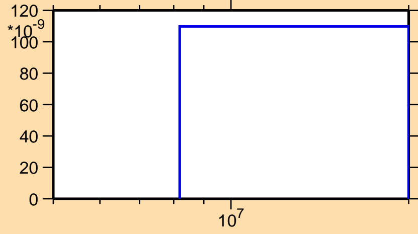
\sigma vs. E for ^{139}\text{Pr}(n,2np)
