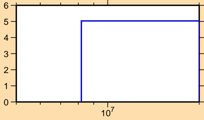
\Delta\sigma/\sigma vs. E for ^{139}\text{Pr}(n,\text{nonel.})
