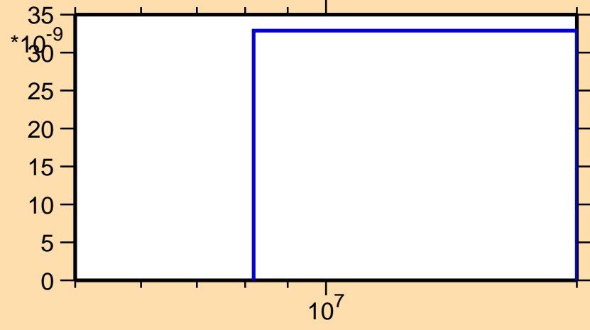
\sigma vs. E for ^{139}\text{Pr}(n,\text{nd})
