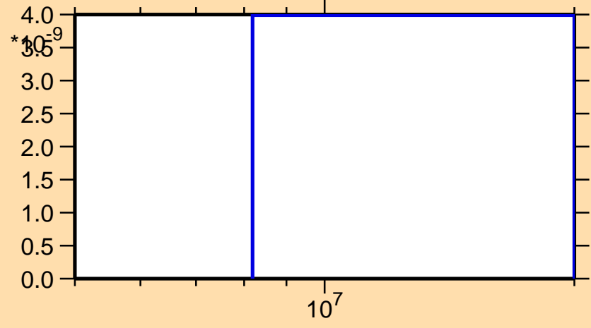
\sigma vs. E for ^{139}\text{Pr}(n,\text{He3})
