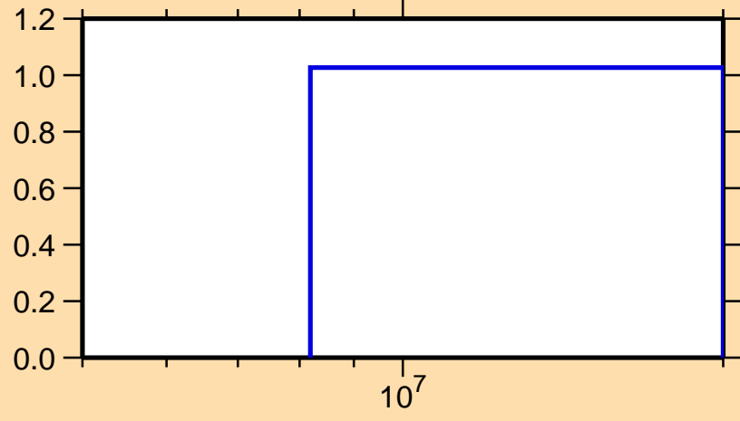
\sigma vs. E for ^{139}\text{Pr}(n,2n)
