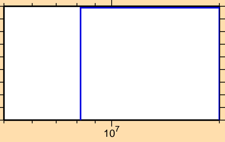
\sigma vs. E for ^{139}\text{Pr}(n,3n)
