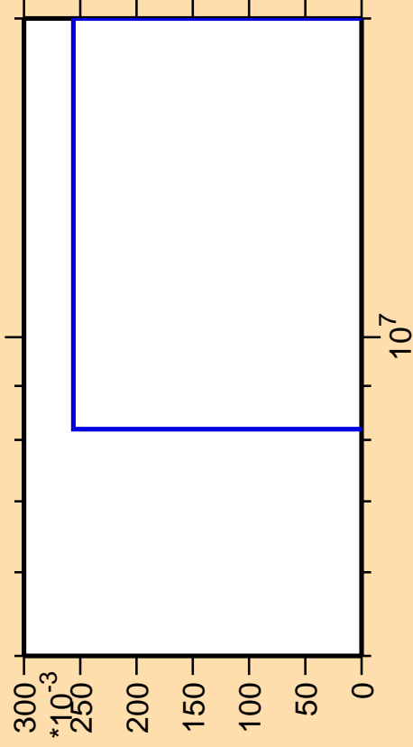
\Delta\sigma/\sigma vs. E for ^{139}\text{Pr}(n,pd)
