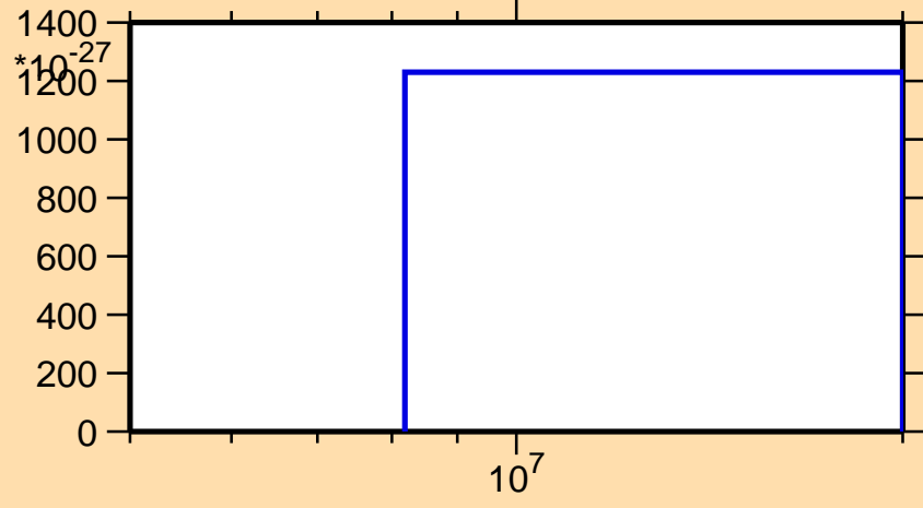
\sigma vs. E for ^{139}\text{Pr}(\text{mt } 11)
