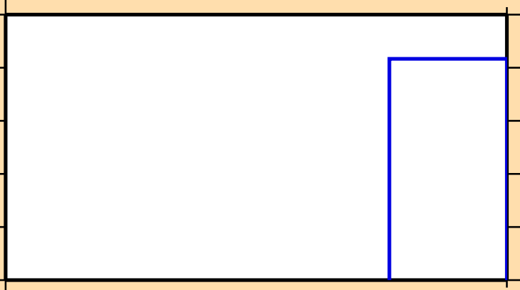
\sigma vs. E for ^{140}\text{Pr}(n,3n)
