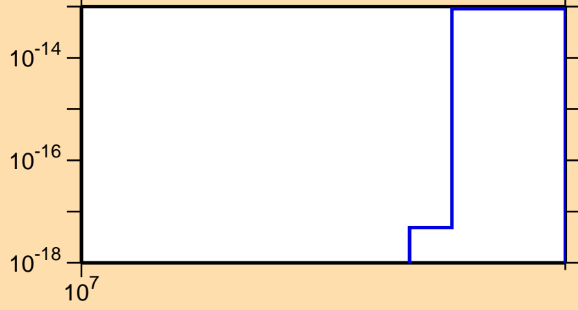
\sigma vs. E for ^{140}\text{Pr}(\text{mt } 34)
