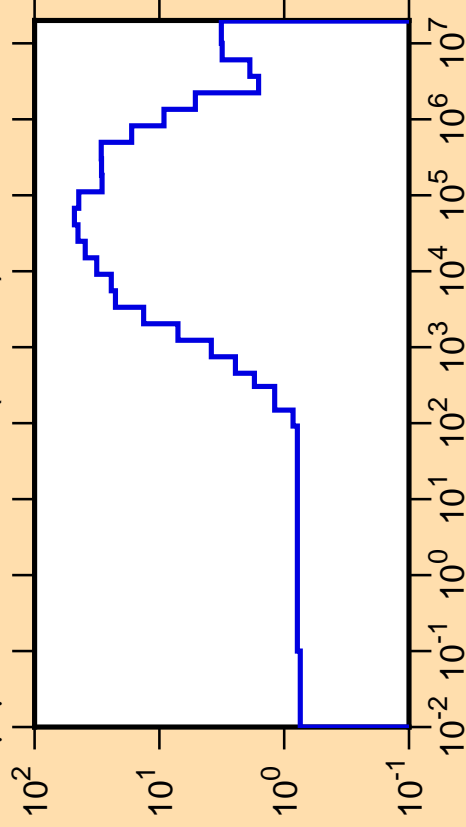
\Delta\mu/\mu vs. E for ^{140}\text{Pr}(\text{mt251})
