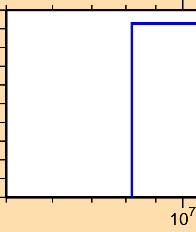
\sigma vs. E for ^{140}\text{Pr}(n,\text{pd})
