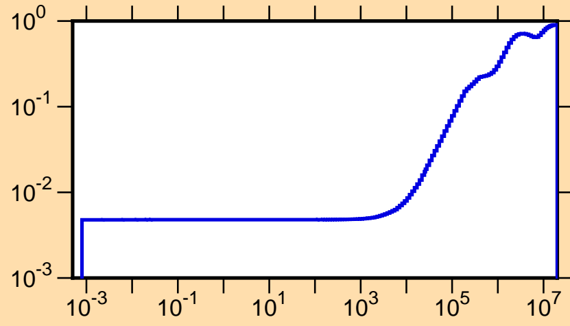
\mu vs. E for ^{141}\text{Pr}(\text{mt251})
