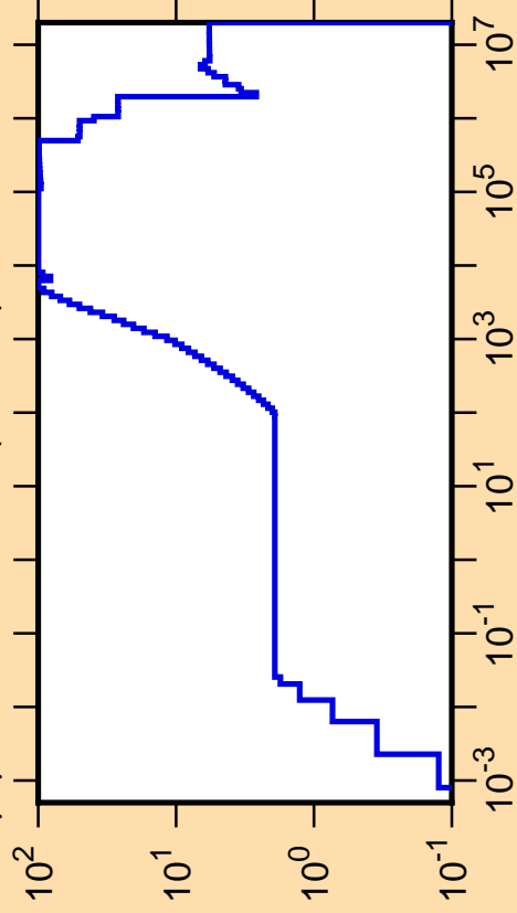
\Delta\mu/\mu vs. E for ^{141}\text{Pr}(\text{mt251})
