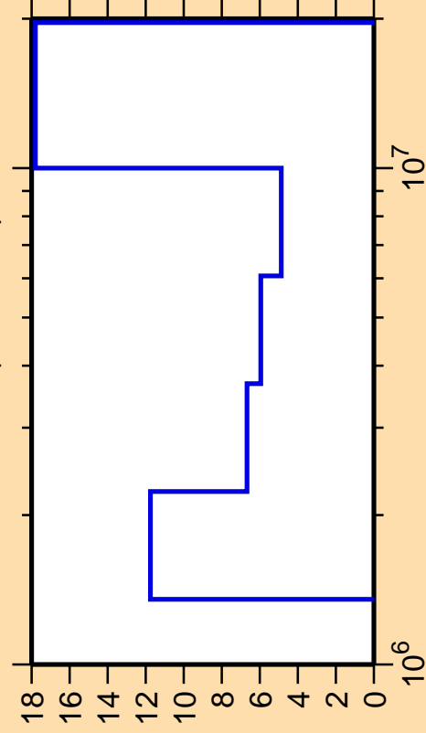
\Delta\sigma/\sigma vs. E for ^{141}\text{Pr}(n, ncont.)
