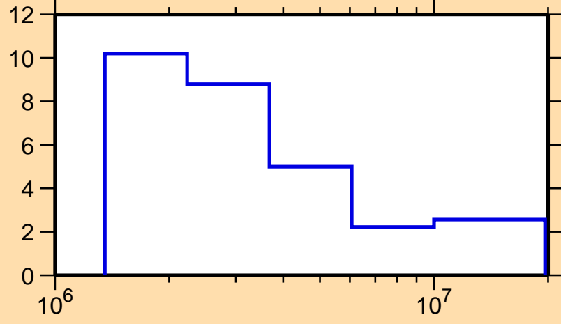
\Delta\sigma/\sigma vs. E for ^{141}\text{Pr}(n, tot.)
