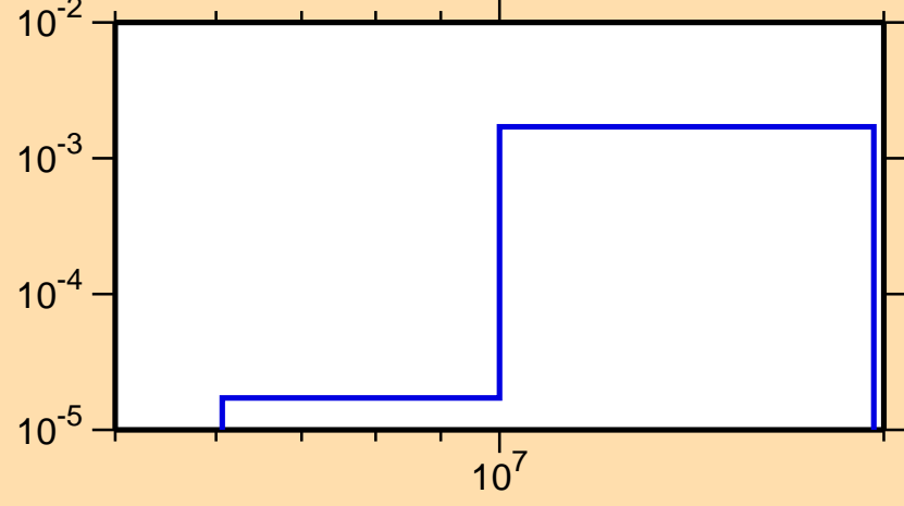
\sigma vs. E for ^{141}\text{Pr}(n,np)
