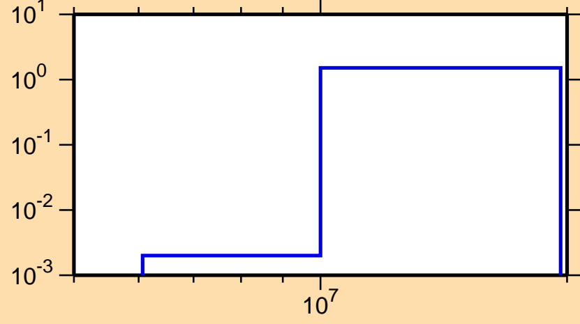
\sigma vs. E for ^{141}\text{Pr}(n,2n)
