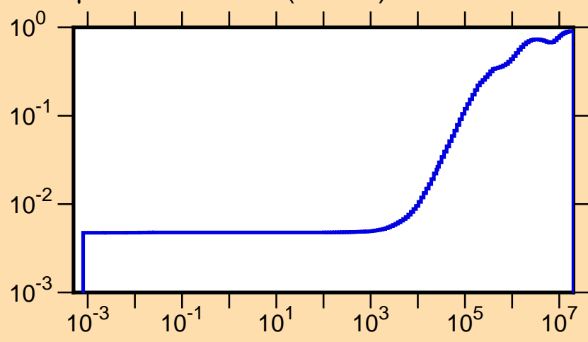
\mu vs. E for ^{142}\text{Pr}(\text{mt251})
