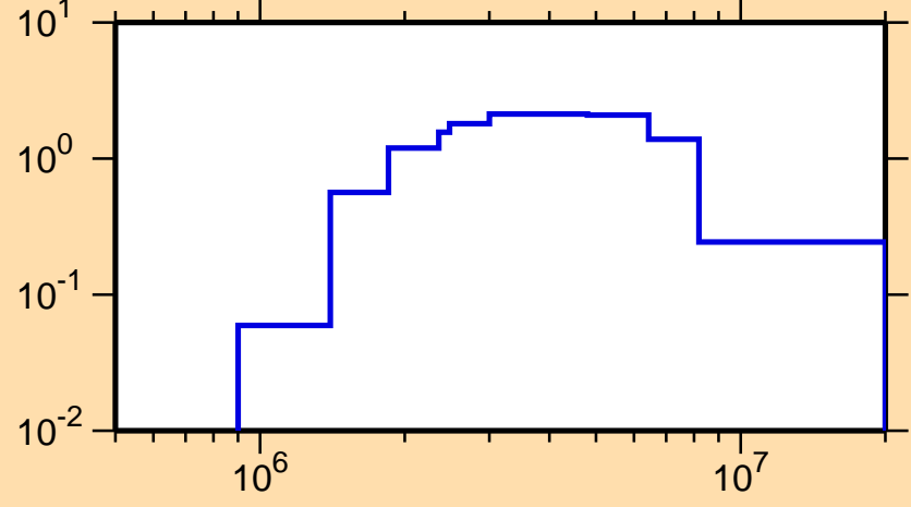
\sigma vs. E for ^{142}\text{Pr}(n,n\text{cont.})
