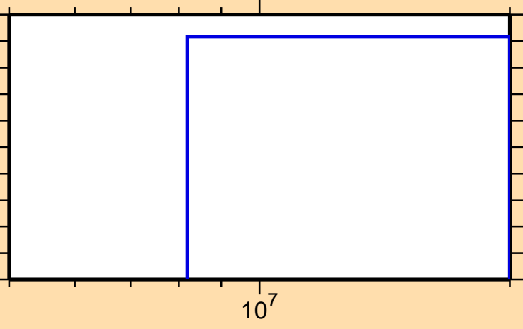
\sigma vs. E for ^{142}\text{Pr}(\text{mt } 34)
