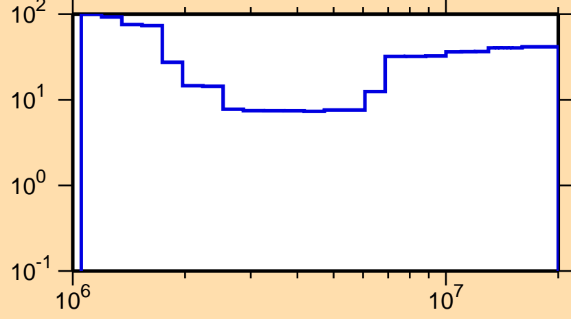
\Delta\sigma/\sigma vs. E for ^{142}\text{Pr}(n,n\text{cont.})
