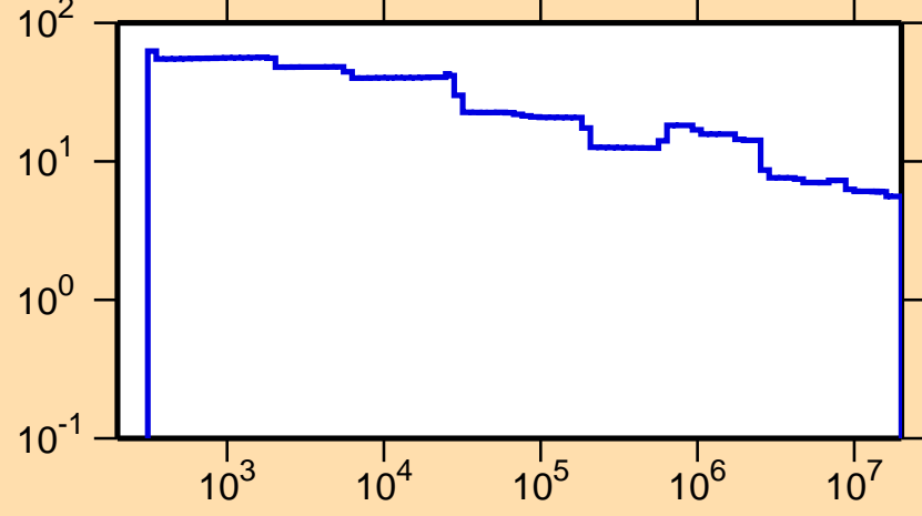
\Delta\sigma/\sigma vs. E for ^{142}\text{Pr}(n,\text{nonel.})
