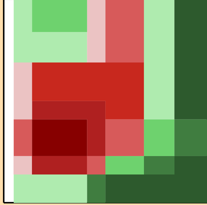
\Delta\sigma/\sigma vs. E for ^{142}\text{Pr}(n,2n)
