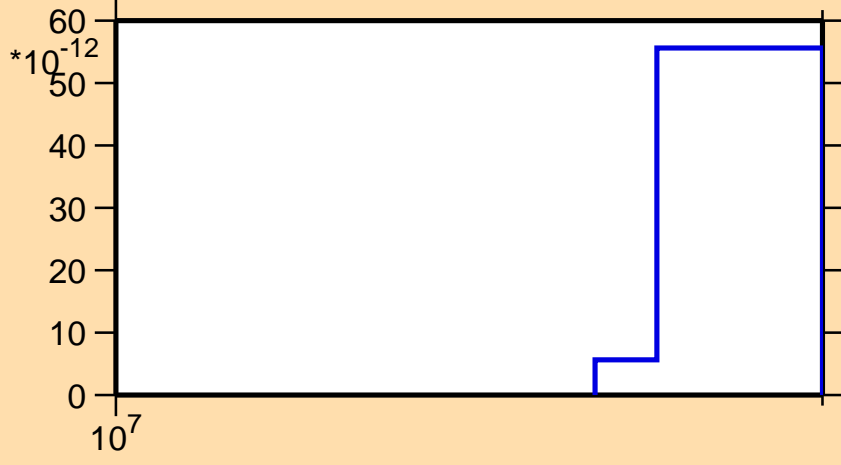
\sigma vs. E for ^{143}\text{Pr} (mt 45)
