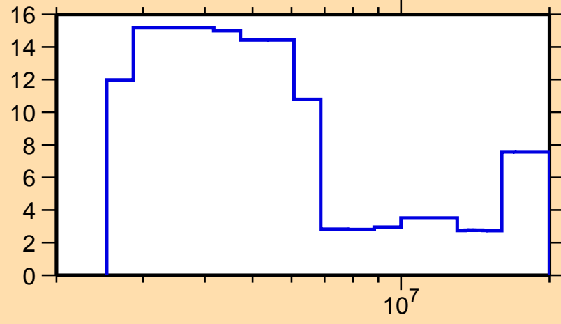
\Delta\sigma/\sigma vs. E for ^{143}\text{Pr}(n, tot.)
