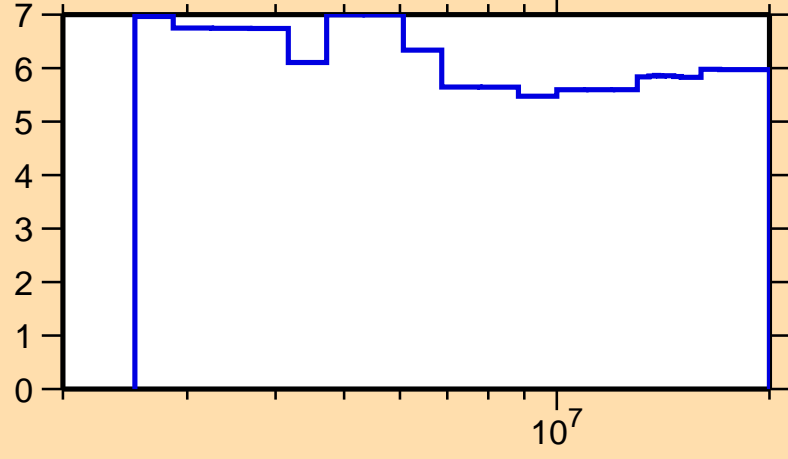
\Delta\sigma/\sigma vs. E for ^{143}\text{Pr}(n,n\text{oncl.})
