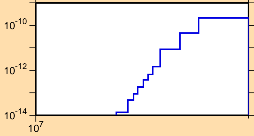
\sigma vs. E for ^{143}\text{Pr}(\text{mt117})
