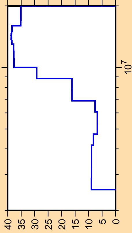
\Delta\sigma/\sigma vs. E for ^{143}\text{Pr}(n, ncont.)
