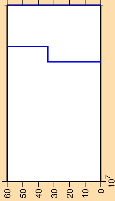
\Delta\sigma/\sigma vs. E for ^{143}\text{Pr} (mt 45)
