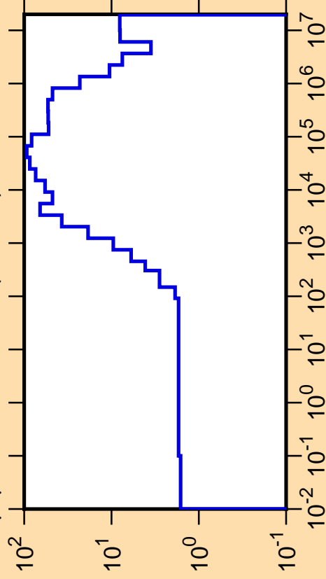
\Delta\mu/\mu vs. E for ^{143}\text{Pr}(\text{mt251})
