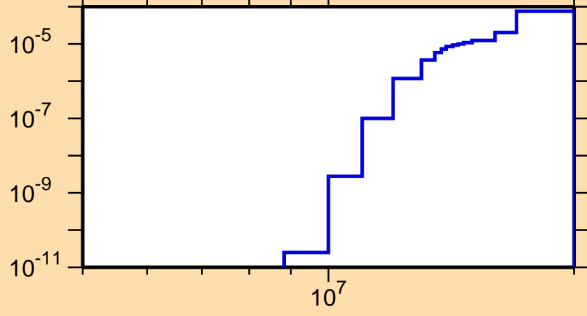
\sigma vs. E for ^{144}\text{Pr}(n,2n\alpha)
