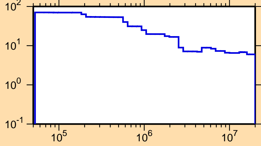
\Delta\sigma/\sigma vs. E for ^{144}\text{Pr}(n,\text{nonel.})
