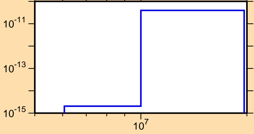
\sigma vs. E for ^{144}\text{Pr}(n,p\alpha)
