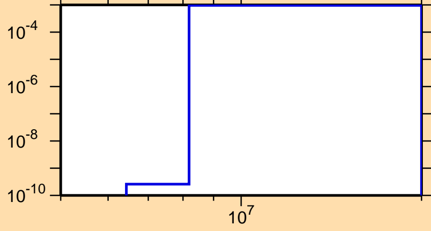
\sigma vs. E for ^{144}\text{Pr}(n,d)
