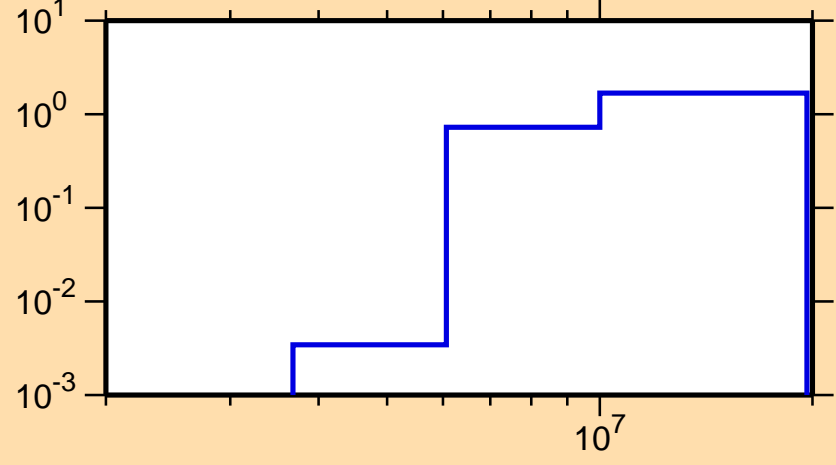
\sigma vs. E for ^{144}\text{Pr}(n,2n)
