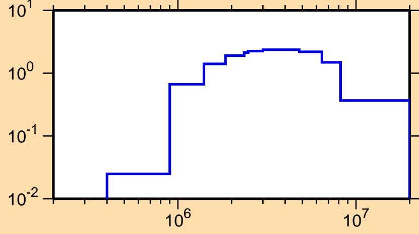
\sigma vs. E for ^{144}\text{Pr}(n,n\text{cont.})
