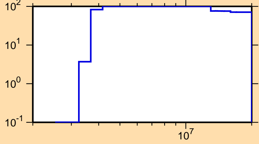
\Delta\sigma/\sigma vs. E for ^{145}\text{Pr}(n,p)
