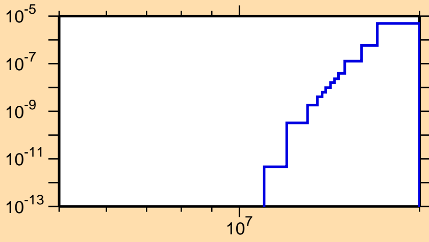
\sigma vs. E for ^{145}\text{Pr}(n,2n\alpha)
