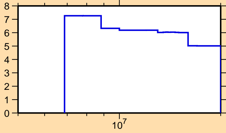
\Delta\sigma/\sigma vs. E for ^{145}\text{Pr}(n,\text{nonel.})
