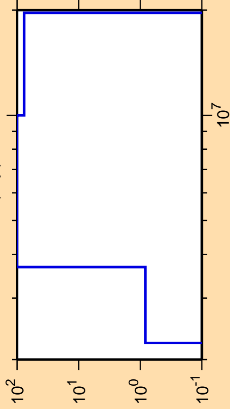
\Delta\sigma/\sigma vs. E for ^{145}\text{Pr}(n,p)
