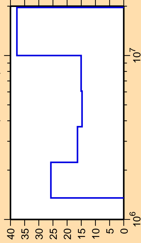
\Delta\sigma/\sigma vs. E for ^{145}\text{Pr}(n, ncont.)
