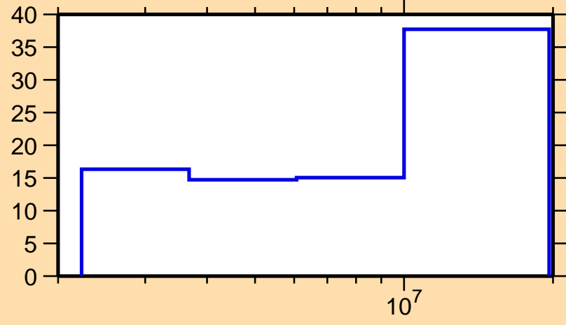
\Delta\sigma/\sigma vs. E for ^{145}\text{Pr}(n,ncont.)
