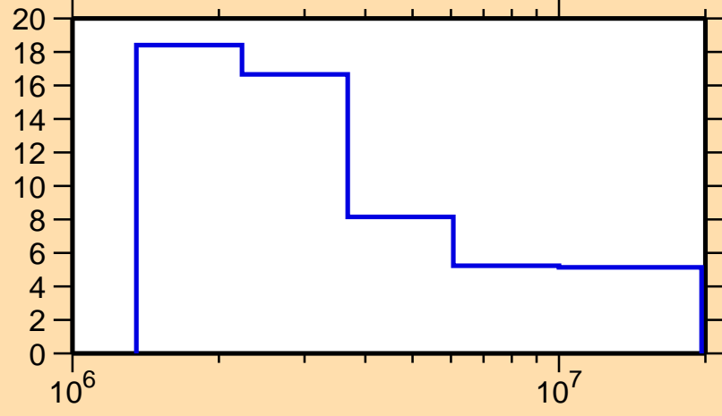
\Delta\sigma/\sigma vs. E for ^{145}\text{Pr}(n, tot.)
