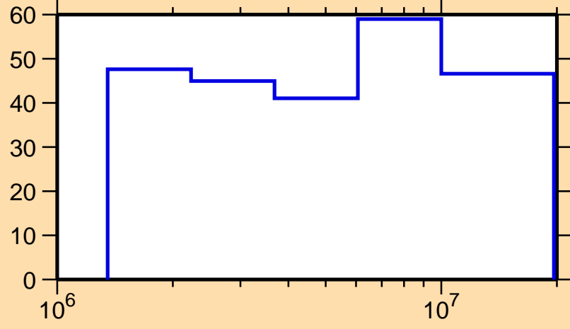
\Delta\sigma/\sigma vs. E for ^{145}\text{Pr}(n,n_1)
