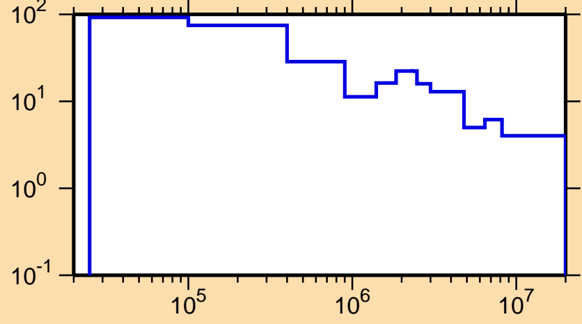
\Delta\sigma/\sigma vs. E for ^{145}\text{Pr}(n,\text{tot.})
