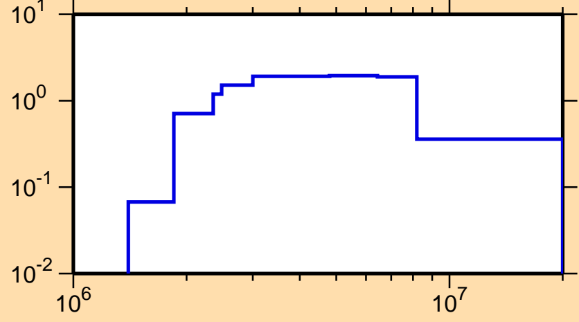
\sigma vs. E for ^{145}\text{Pr}(n,n\text{cont.})
