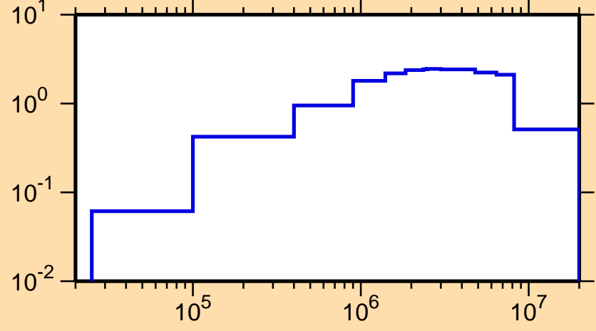
\sigma vs. E for ^{145}\text{Pr}(n,\text{inel.})
