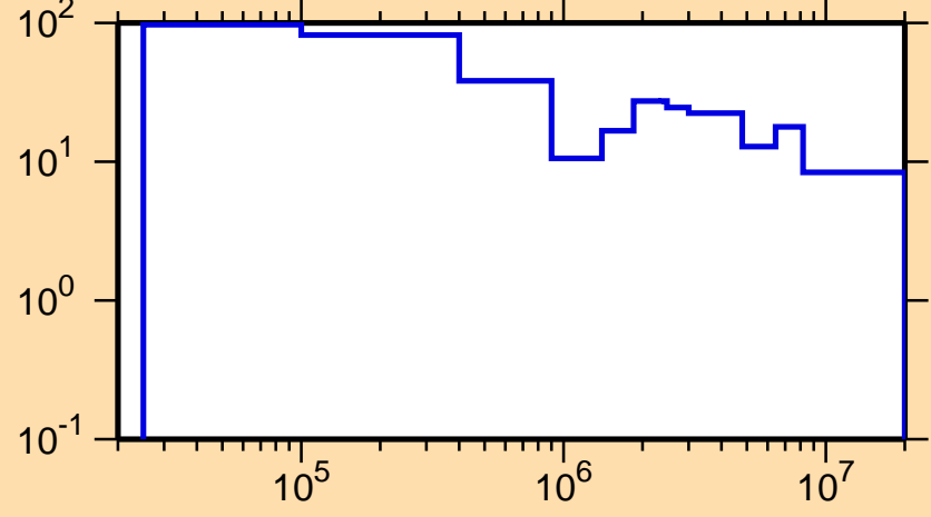
\Delta\sigma/\sigma vs. E for ^{145}\text{Pr}(n,\text{el.})
