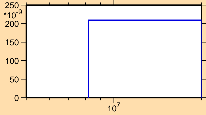
\sigma vs. E for ^{145}\text{Pr}(n,\text{nd})
