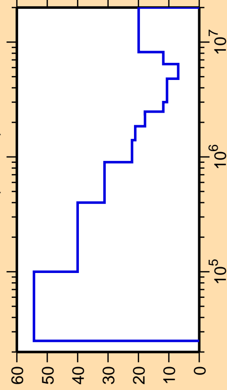
\Delta\sigma/\sigma vs. E for ^{145}\text{Pr}(n,\text{inel.})
