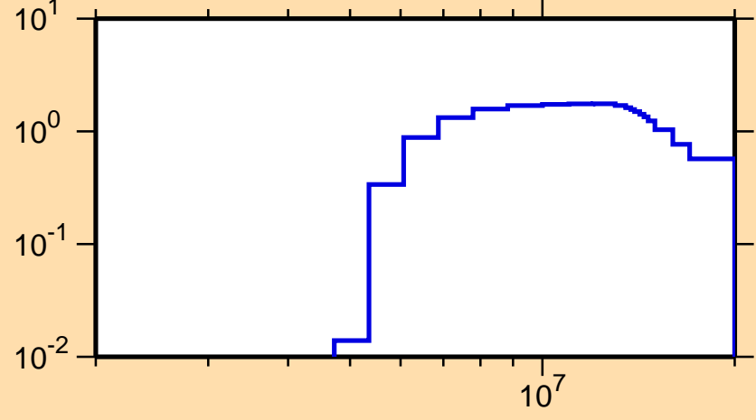
\sigma vs. E for ^{146}\text{Pr}(n,2n)
