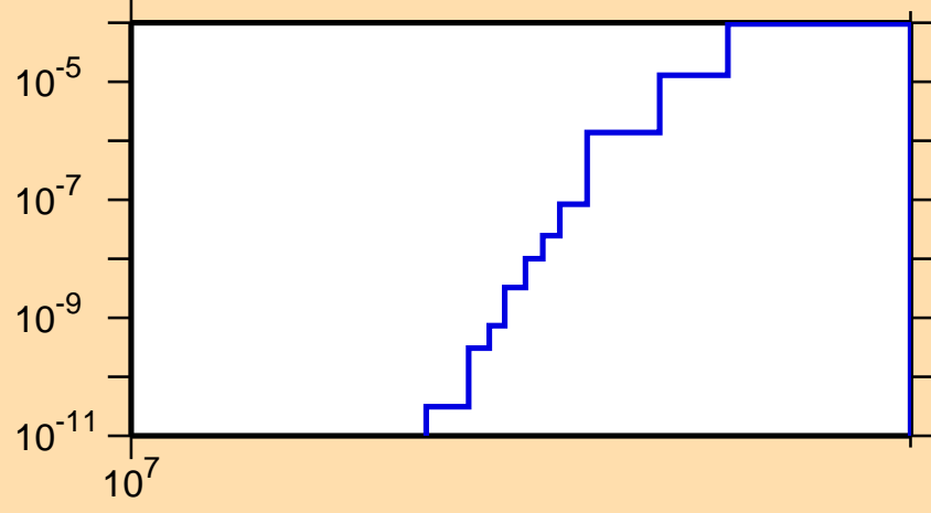
\sigma vs. E for ^{146}\text{Pr}(n,nt)
