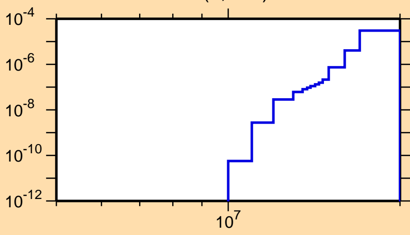
\sigma vs. E for ^{146}\text{Pr}(n,2n\alpha)
