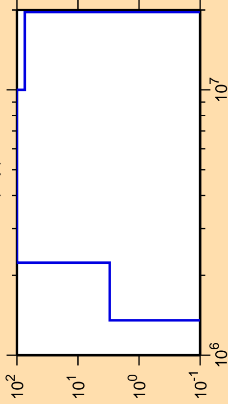
\Delta\sigma/\sigma vs. E for ^{146}\text{Pr}(n,p)
