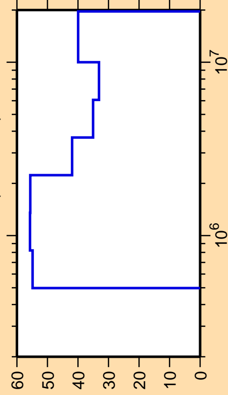
\Delta\sigma/\sigma vs. E for ^{146}\text{Pr}(n,\text{ncont.})
