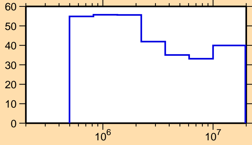
\Delta\sigma/\sigma vs. E for ^{146}\text{Pr}(n,n\text{cont.})
