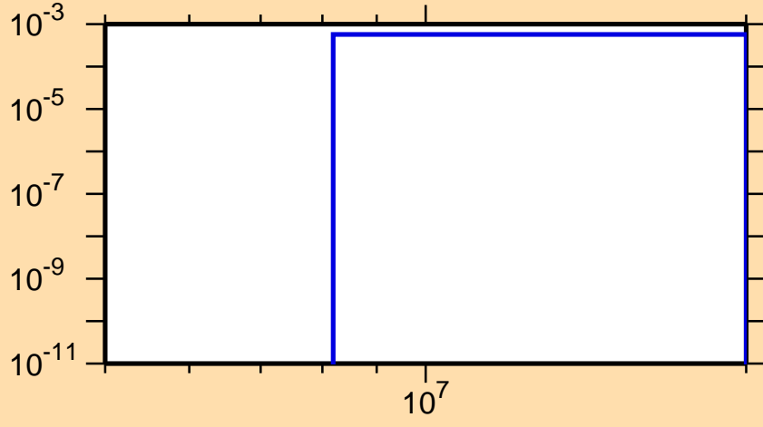
\sigma vs. E for ^{146}\text{Pr}(n,np)
