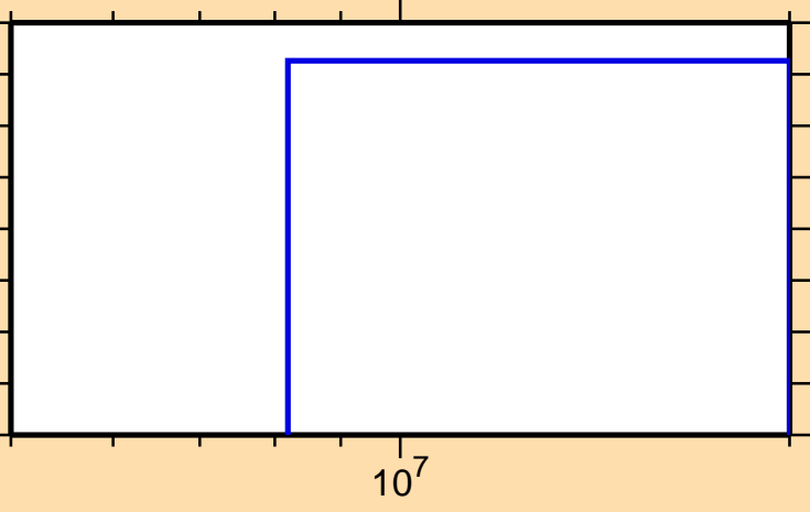
\sigma vs. E for ^{146}\text{Pr}(n,nt)
