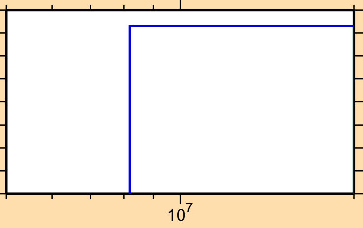
\sigma vs. E for ^{146}\text{Pr}(n,3n\alpha)
