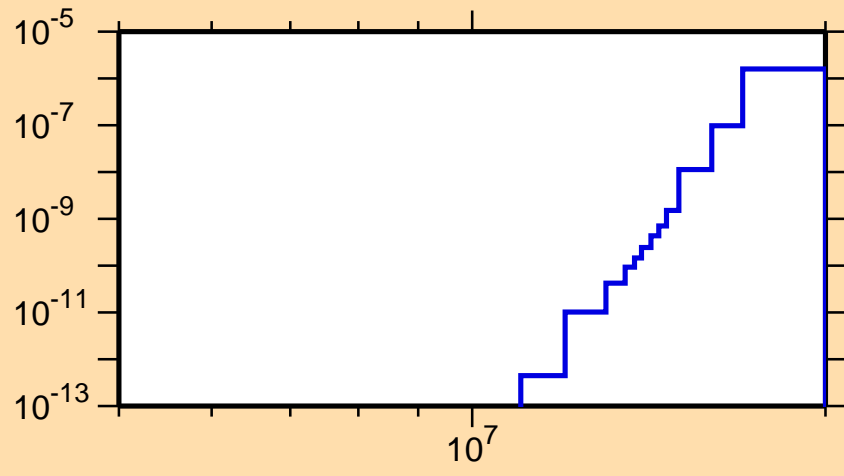
\sigma vs. E for ^{147}\text{Pr}(n,2n\alpha)
