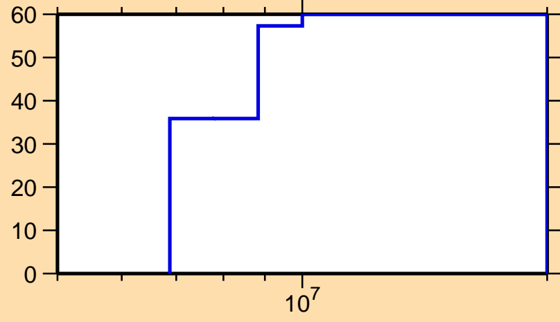
\Delta\sigma/\sigma vs. E for ^{147}\text{Pr}(n,\text{inel.})
