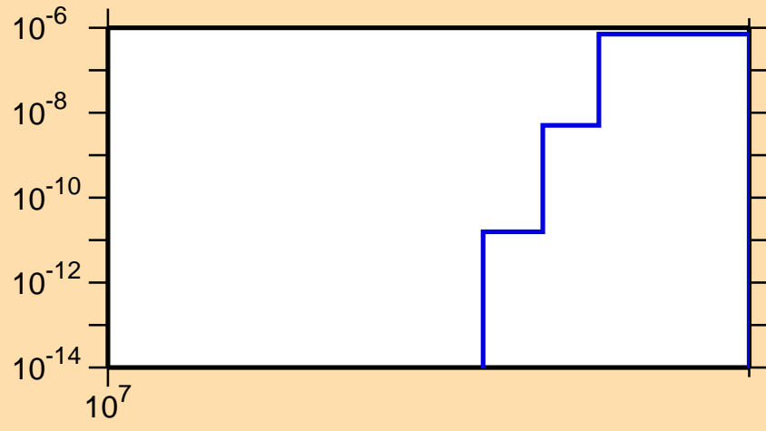
\sigma vs. E for ^{147}\text{Pr}(n,2np)
