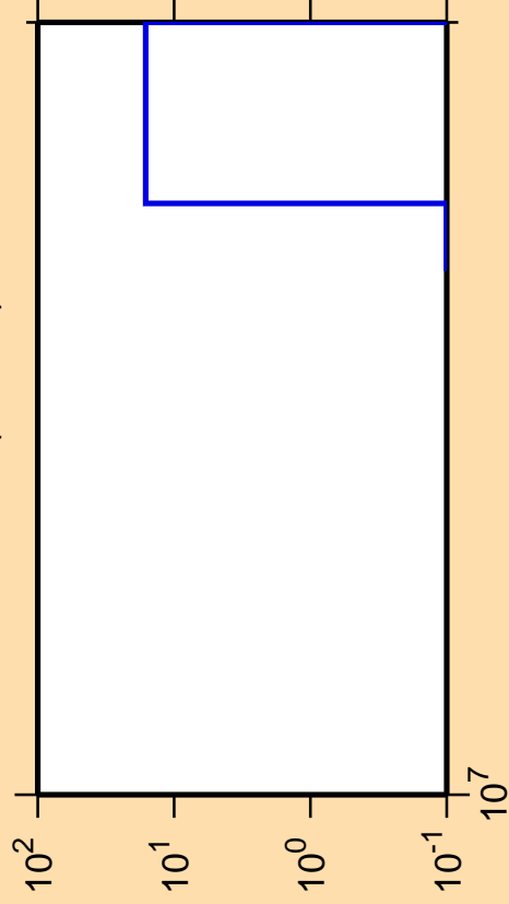
\Delta\sigma/\sigma vs. E for ^{147}\text{Pr}(n,\text{He3})
