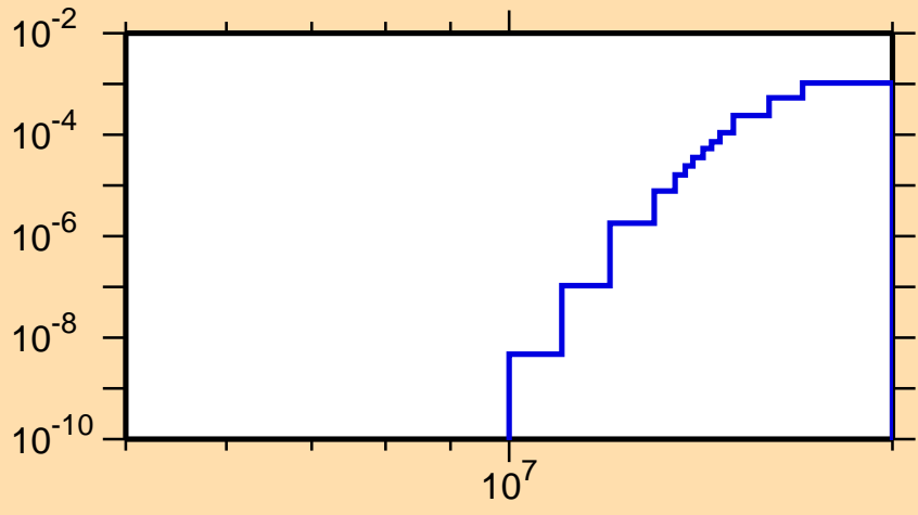
\sigma vs. E for ^{147}\text{Pr}(n,t)
