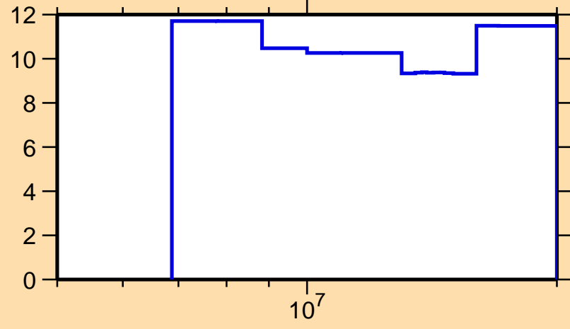
\Delta\sigma/\sigma vs. E for ^{147}\text{Pr}(n,\text{nonel.})
