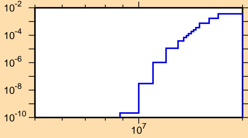
\sigma vs. E for ^{147}\text{Pr}(n,np)
