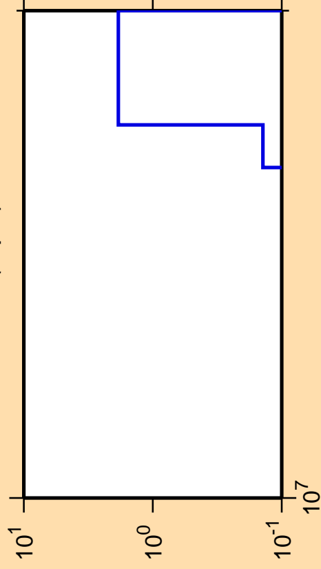
\Delta\sigma/\sigma vs. E for ^{147}\text{Pr}(n,p\alpha)
