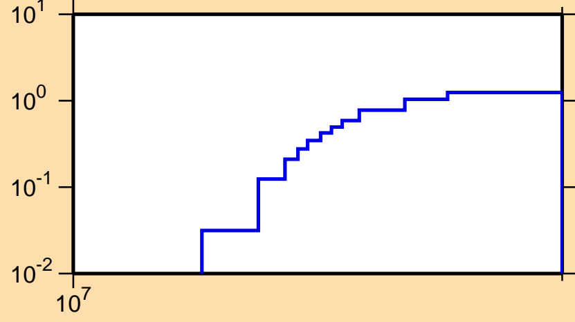
\sigma vs. E for ^{147}\text{Pr}(n,3n)
