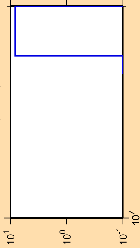
\Delta\sigma/\sigma vs. E for ^{147}\text{Pr}(\text{mt } 11)
