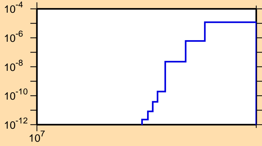
\sigma vs. E for ^{147}\text{Pr}(n,nd)
