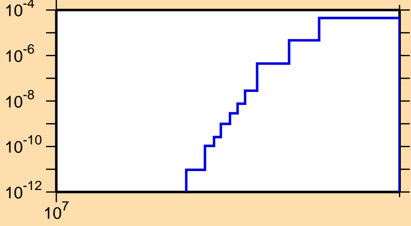
\sigma vs. E for ^{147}\text{Pr}(n,nt)
