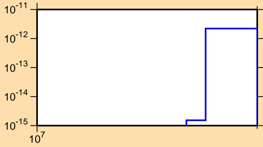
\sigma vs. E for ^{147}\text{Pr}(n,\text{He3})
