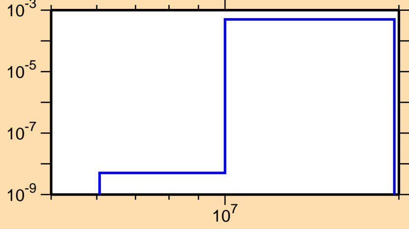
\sigma vs. E for ^{147}\text{Pr}(n,d)
