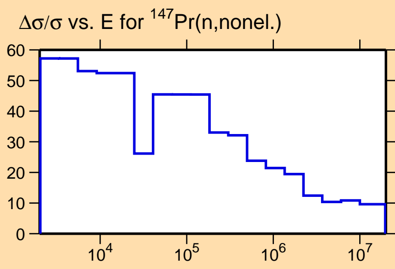
\Delta\sigma/\sigma vs. E for ^{147}\text{Pr}(n,\text{nonel.})
