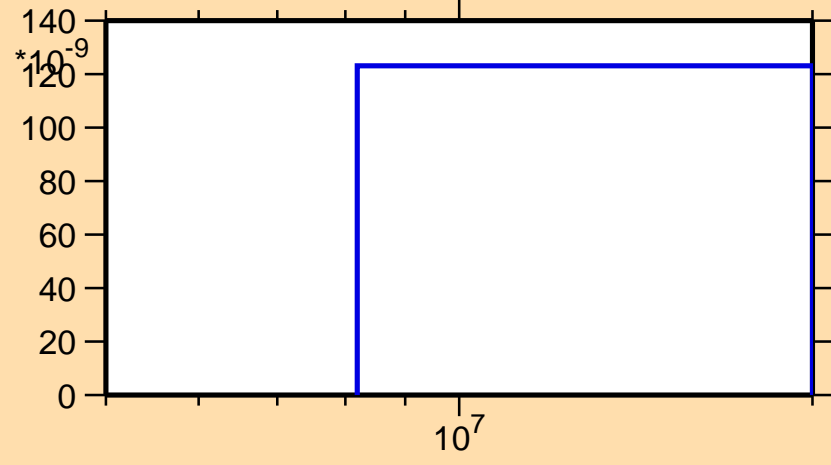
\sigma vs. E for ^{147}\text{Pr}(n,\text{nd})
