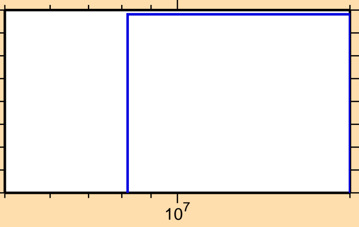
\sigma vs. E for ^{147}\text{Pr}(n,t)
