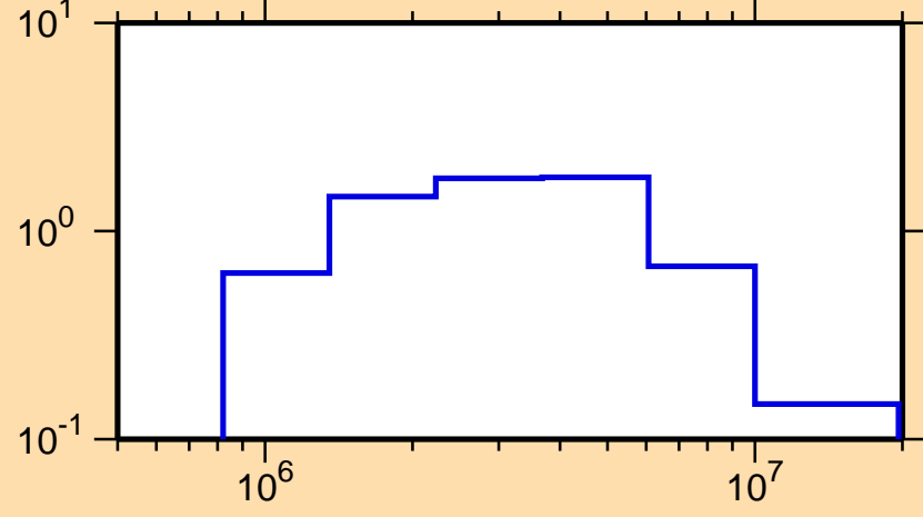
\sigma vs. E for ^{148}\text{Pr}(n,n\text{cont.})
