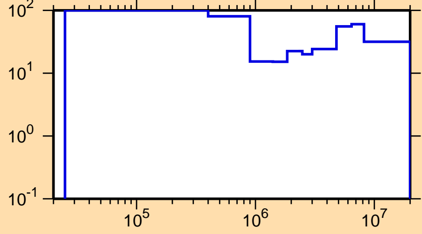
\Delta\sigma/\sigma vs. E for ^{148}\text{Pr}(n,\text{el.})
