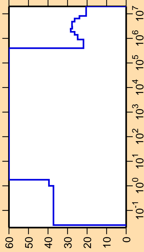
\Delta\sigma/\sigma vs. E for ^{148}\text{Pr}(n,\text{nonel.})
