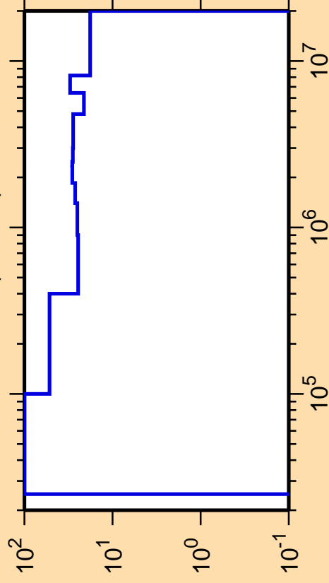
\Delta\sigma/\sigma vs. E for ^{148}\text{Pr}(n,\text{inel.})
