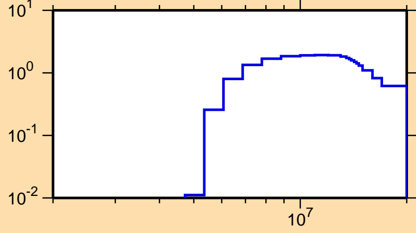
\sigma vs. E for ^{148}\text{Pr}(n,2n)
