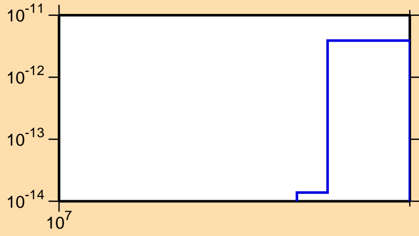
\sigma vs. E for ^{148}\text{Pr}(n,3n\alpha)
