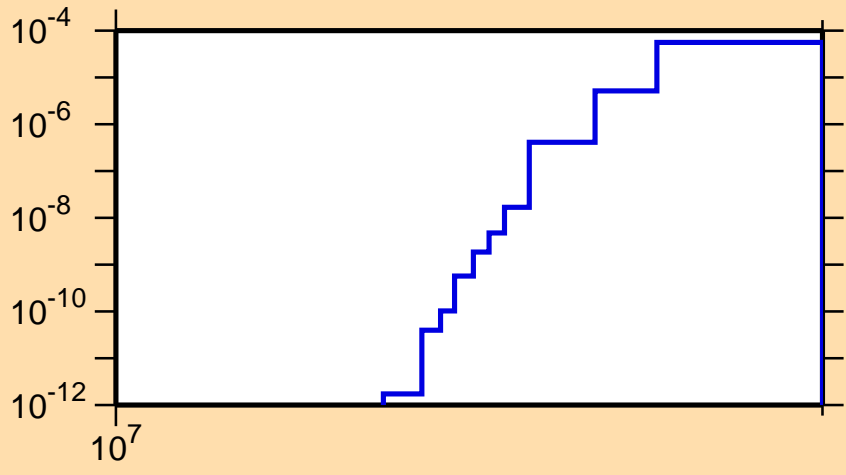
\sigma vs. E for ^{148}\text{Pr}(n,nt)
