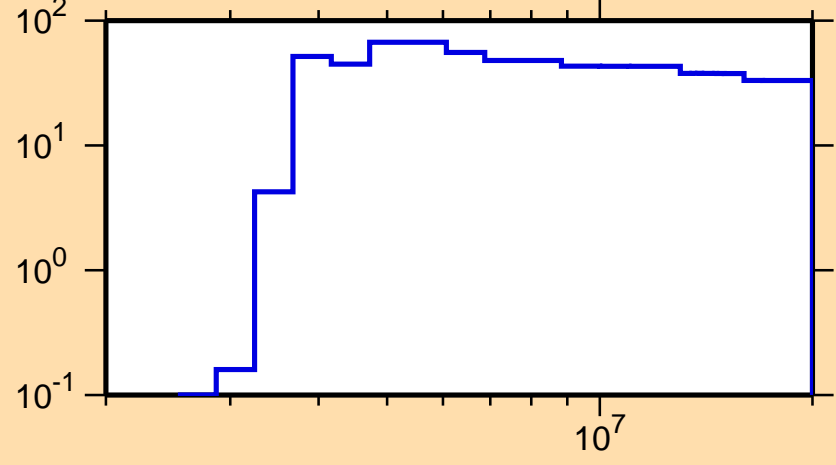
\Delta\sigma/\sigma vs. E for ^{148}\text{Pr}(n,p)
