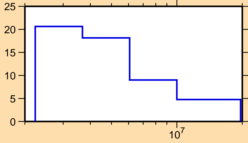
\Delta\sigma/\sigma vs. E for ^{148}\text{Pr}(n,el.)
