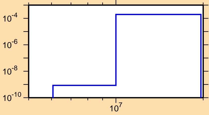
\sigma vs. E for ^{148}\text{Pr}(n,\alpha)
