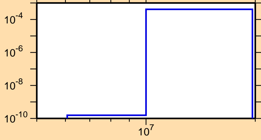
\sigma vs. E for ^{148}\text{Pr}(n,d)
