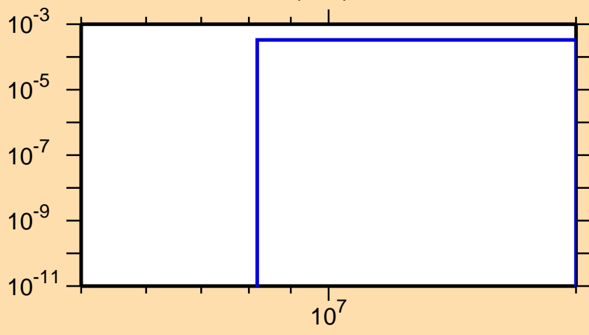
\sigma vs. E for ^{148}\text{Pr}(n,d)
