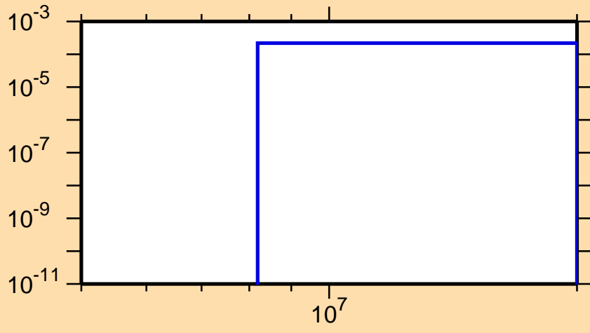
\sigma vs. E for ^{148}\text{Pr}(n,np)
