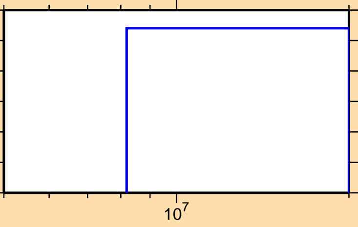
\sigma vs. E for ^{148}\text{Pr}(n,\text{nd})
