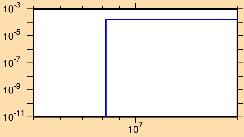
\sigma vs. E for ^{148}\text{Pr}(n,t)
