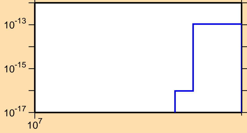
\sigma vs. E for ^{149}\text{Pr}(\text{mt } 11)
