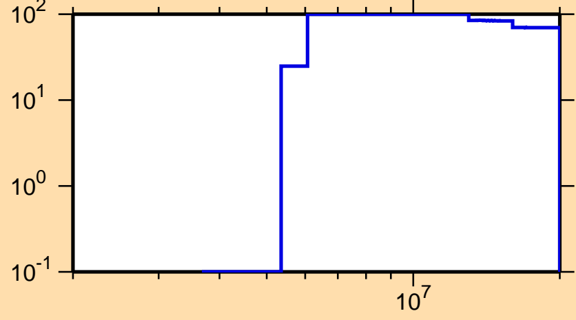
\Delta\sigma/\sigma vs. E for ^{149}\text{Pr}(n,p)
