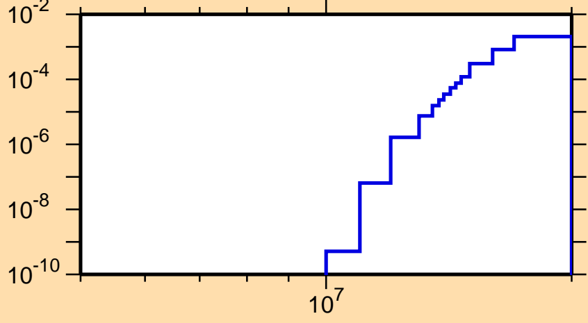
\sigma vs. E for ^{149}\text{Pr}(n,np)
