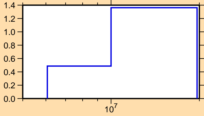
\sigma vs. E for ^{149}\text{Pr}(n,2n)
