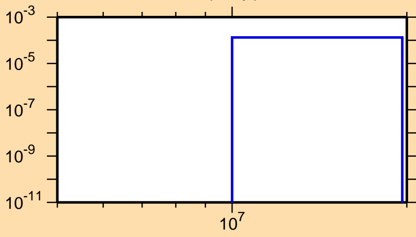
\sigma vs. E for ^{149}\text{Pr}(n,np)
