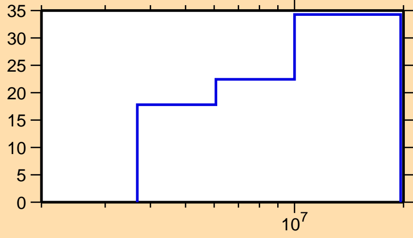
\Delta\sigma/\sigma vs. E for ^{149}\text{Pr}(n,ncont.)
