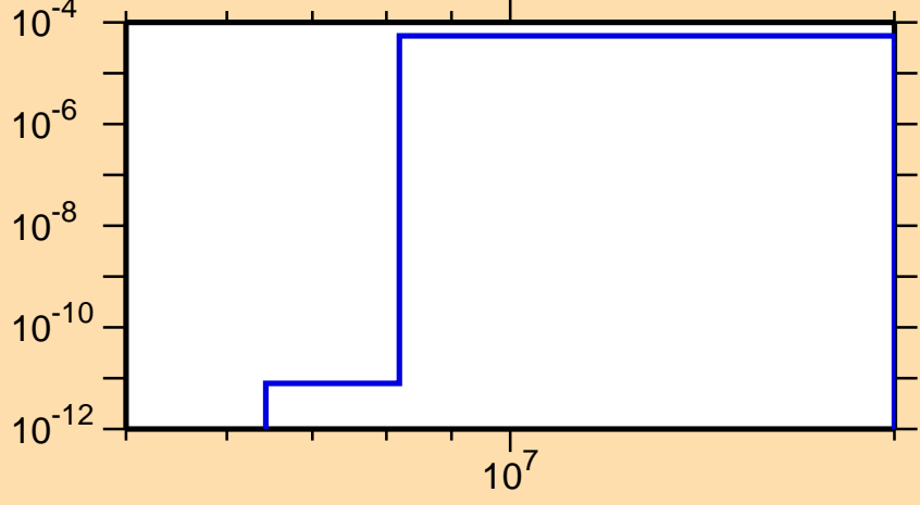
\sigma vs. E for ^{149}\text{Pr}(n,\alpha)
