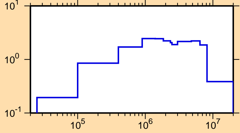
\sigma vs. E for ^{149}\text{Pr}(n,\text{inel.})
